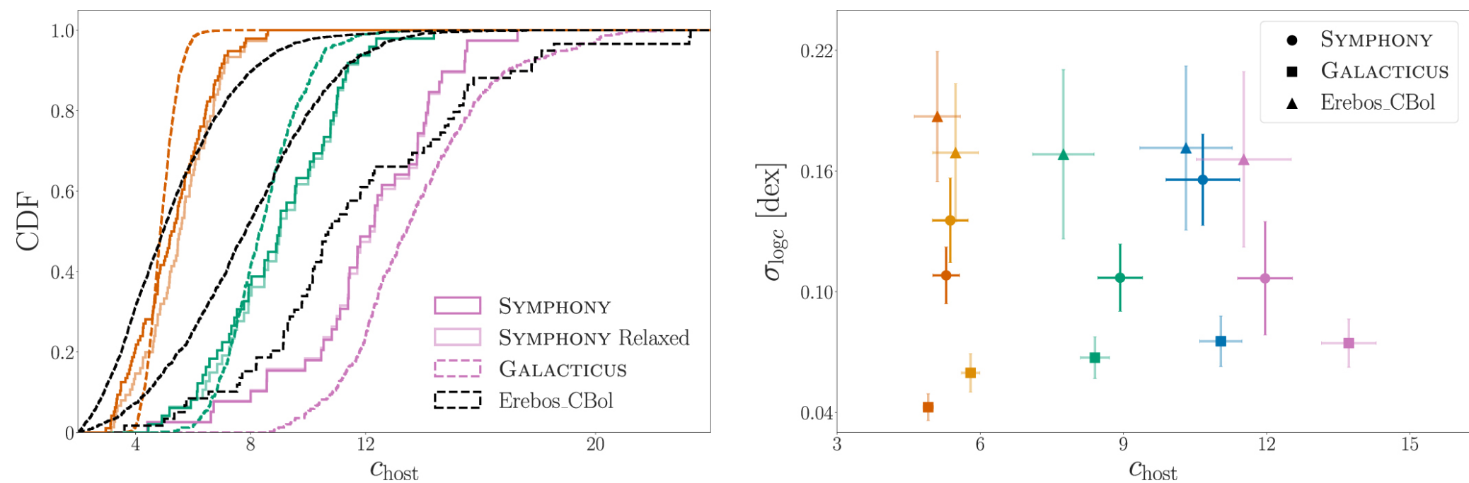
Figure 9. from Ethan O. Nadler et al 2023 Astrophys. J. 945 doi:10.3847/1538-4357/acb68c https://dx.doi.org/10.3847/1538-4357/acb68c © 2023. The Author(s). Published by the American Astronomical Society.
