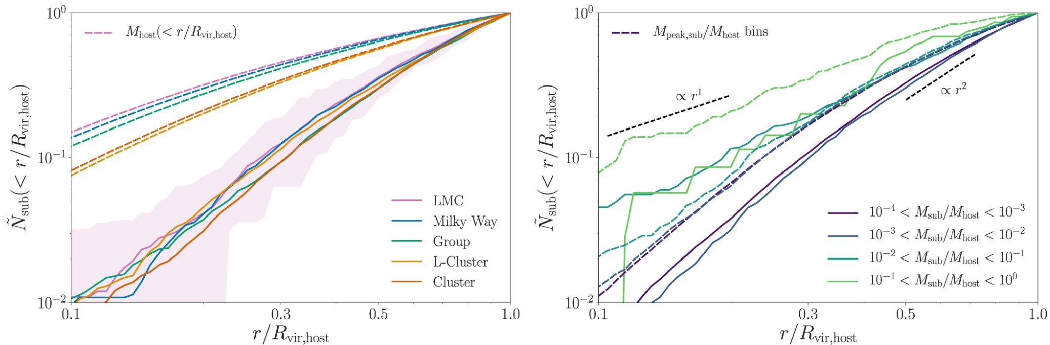
Figure 8. from Ethan O. Nadler et al 2023 Astrophys. J. 945 doi:10.3847/1538-4357/acb68c https://dx.doi.org/10.3847/1538-4357/acb68c © 2023. The Author(s). Published by the American Astronomical Society.
