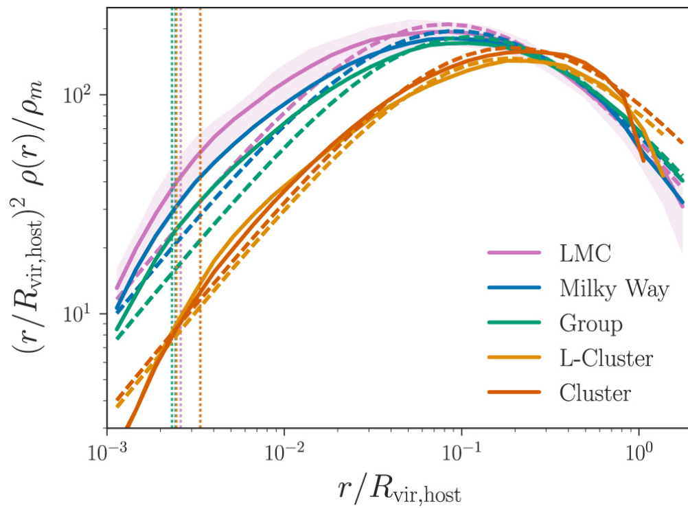
Figure 6. from Ethan O. Nadler et al 2023 Astrophys. J. 945 doi:10.3847/1538-4357/acb68c https://dx.doi.org/10.3847/1538-4357/acb68c © 2023. The Author(s). Published by the American Astronomical Society.
