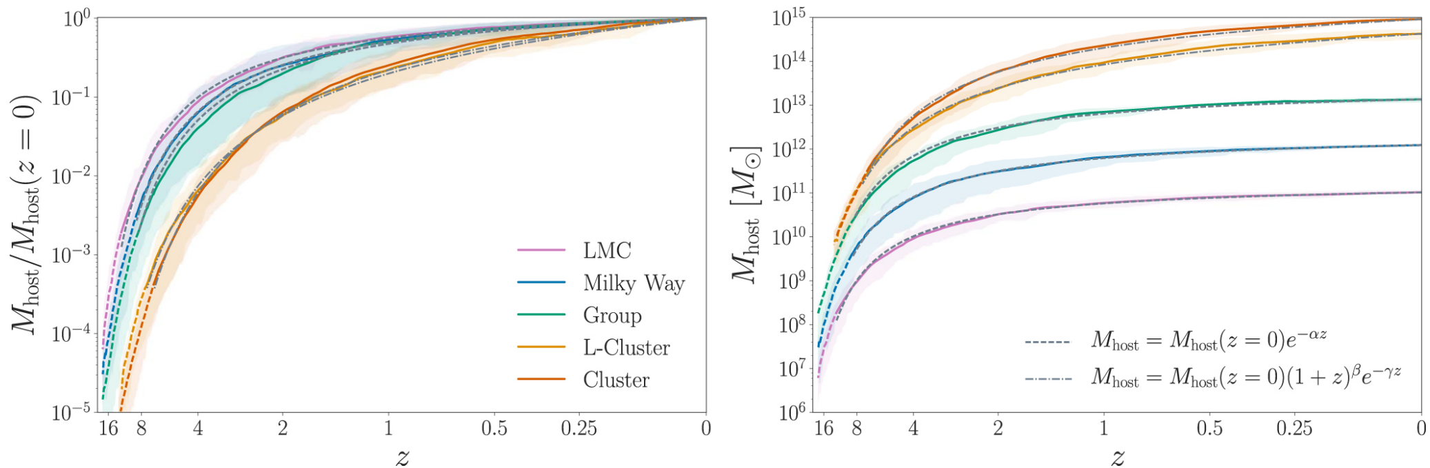
Figure 5. from Ethan O. Nadler et al 2023 Astrophys. J. 945 doi:10.3847/1538-4357/acb68c https://dx.doi.org/10.3847/1538-4357/acb68c © 2023. The Author(s). Published by the American Astronomical Society.
