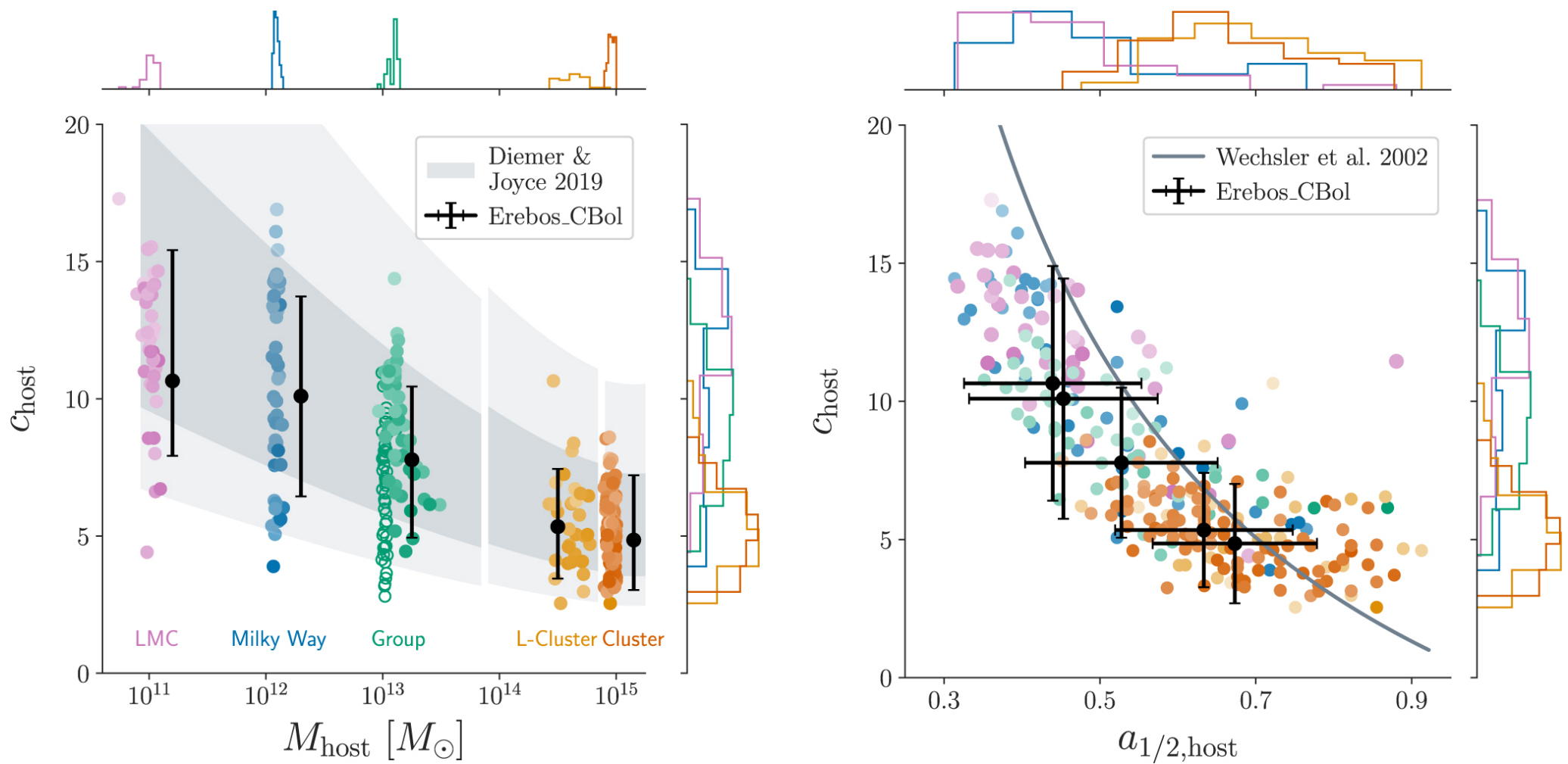
Figure 3. from Ethan O. Nadler et al 2023 Astrophys. J. 945 doi:10.3847/1538-4357/acb68c https://dx.doi.org/10.3847/1538-4357/acb68c © 2023. The Author(s). Published by the American Astronomical Society.
