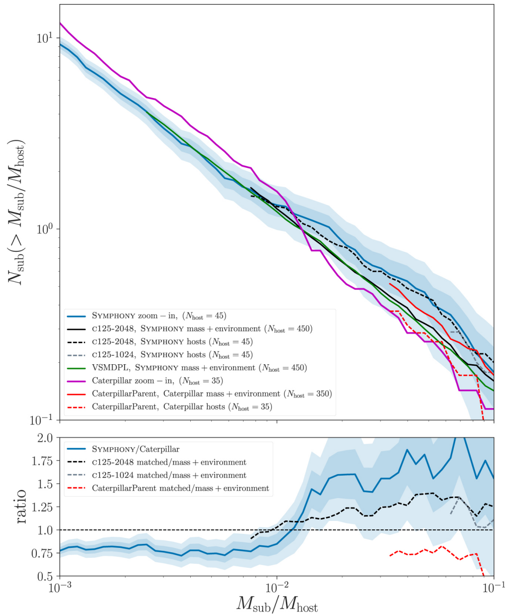
Figure 20. from Ethan O. Nadler et al 2023 Astrophys. J. 945 doi:10.3847/1538-4357/acb68c https://dx.doi.org/10.3847/1538-4357/acb68c © 2023. The Author(s). Published by the American Astronomical Society.
