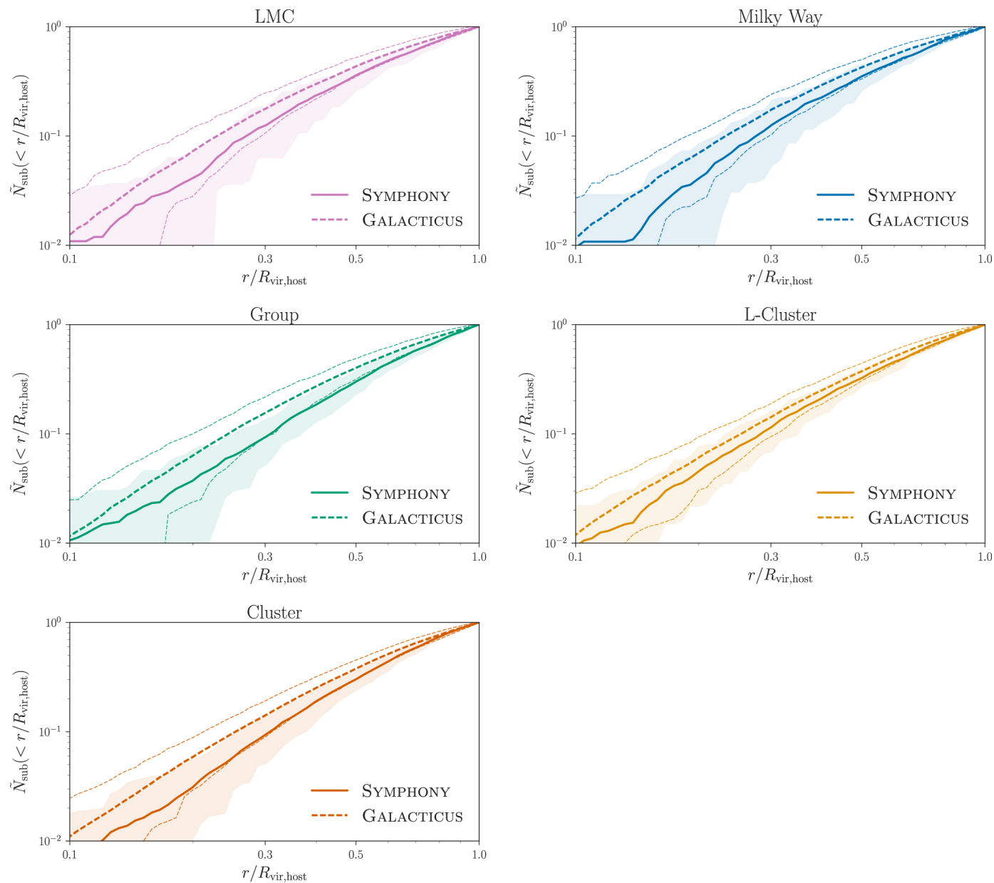
Figure 19. from Ethan O. Nadler et al 2023 Astrophys. J. 945 doi:10.3847/1538-4357/acb68c https://dx.doi.org/10.3847/1538-4357/acb68c © 2023. The Author(s). Published by the American Astronomical Society.
