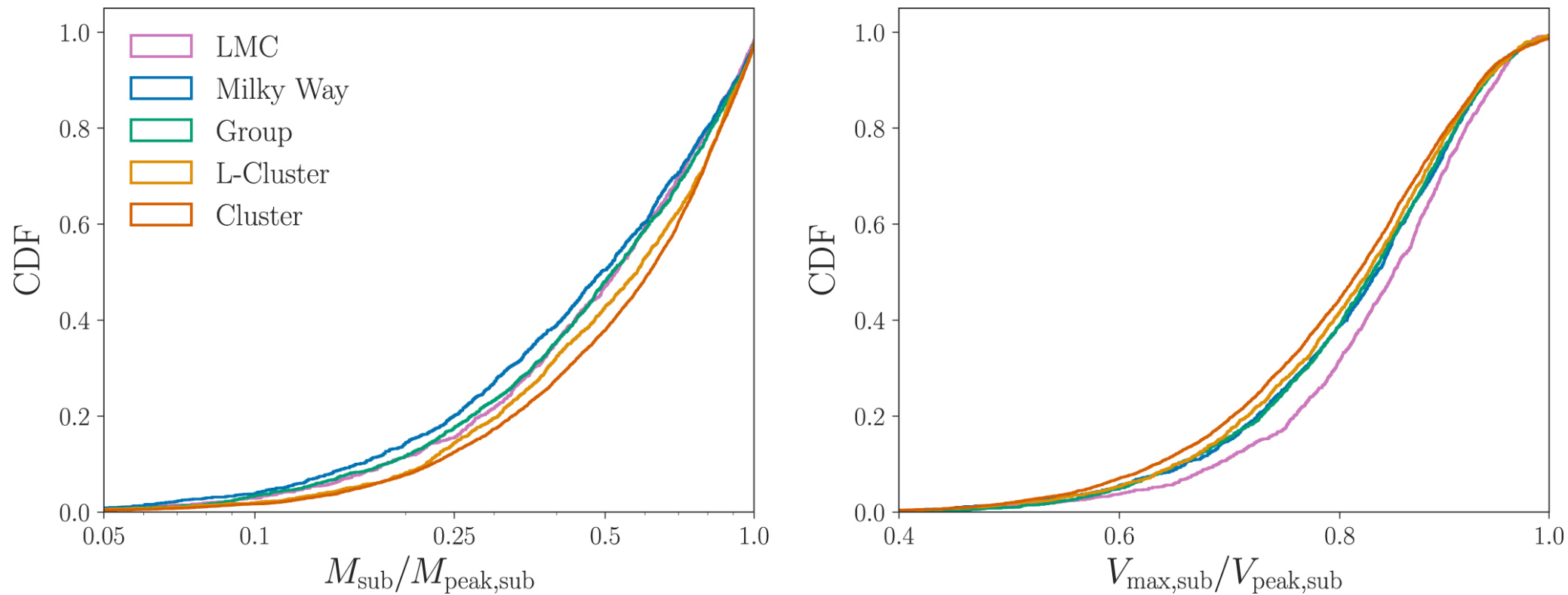
Figure 16. from Ethan O. Nadler et al 2023 Astrophys. J. 945 doi:10.3847/1538-4357/acb68c https://dx.doi.org/10.3847/1538-4357/acb68c © 2023. The Author(s). Published by the American Astronomical Society.
