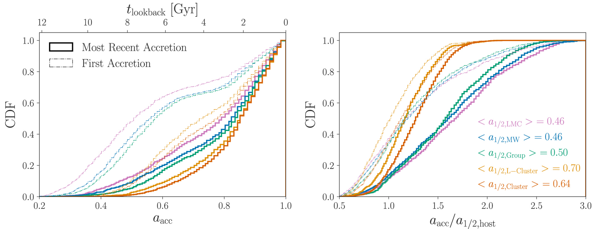
Figure 15. from Ethan O. Nadler et al 2023 Astrophys. J. 945 doi:10.3847/1538-4357/acb68c https://dx.doi.org/10.3847/1538-4357/acb68c © 2023. The Author(s). Published by the American Astronomical Society.
