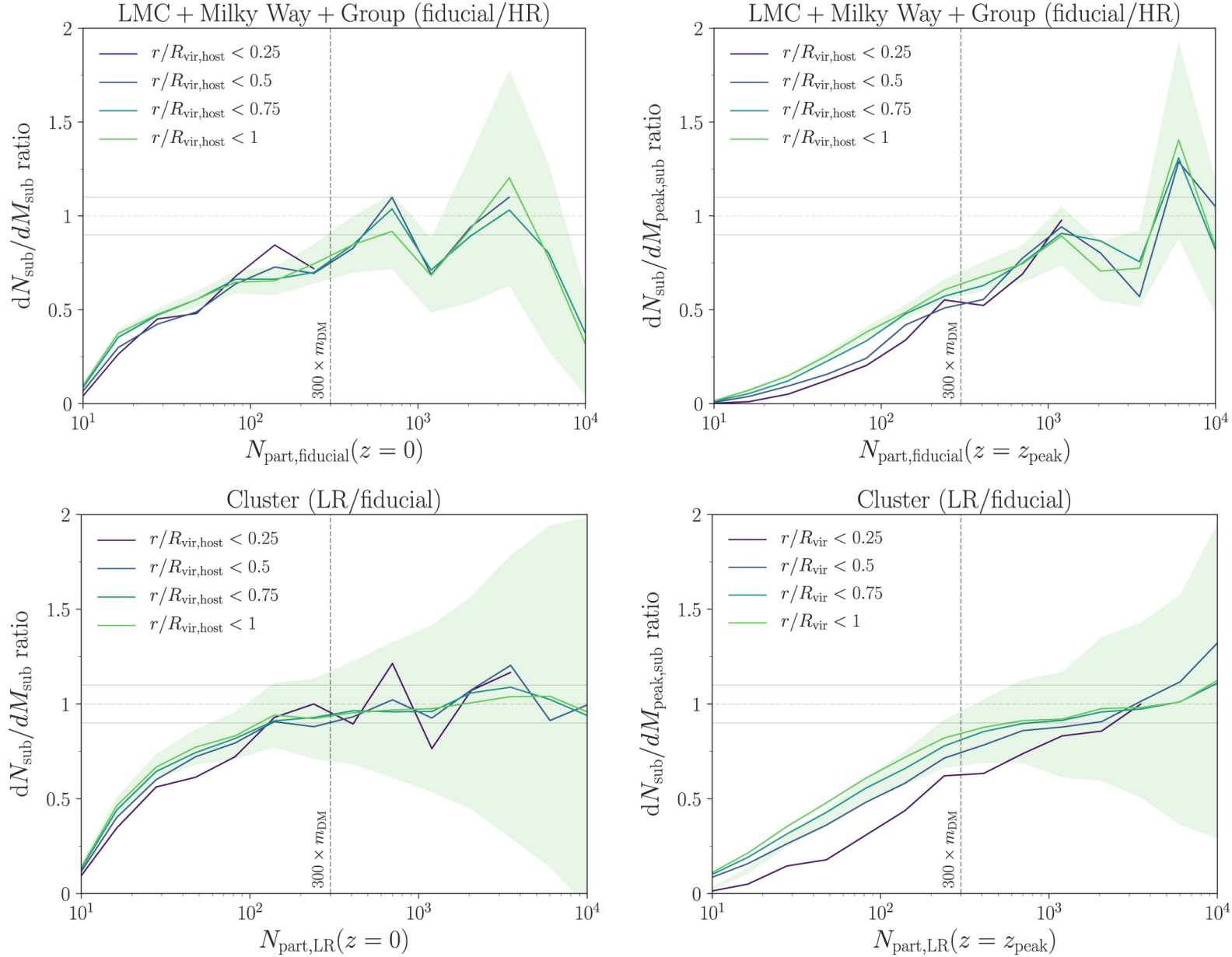
Figure 13. from Ethan O. Nadler et al 2023 Astrophys. J. 945 doi:10.3847/1538-4357/acb68c https://dx.doi.org/10.3847/1538-4357/acb68c © 2023. The Author(s). Published by the American Astronomical Society.
