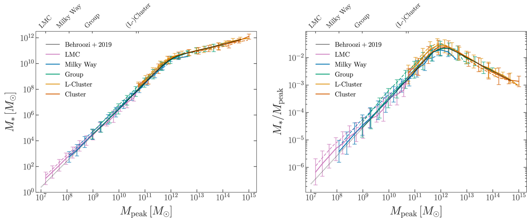
Figure 12. from Ethan O. Nadler et al 2023 Astrophys. J. 945 doi:10.3847/1538-4357/acb68c https://dx.doi.org/10.3847/1538-4357/acb68c © 2023. The Author(s). Published by the American Astronomical Society.
