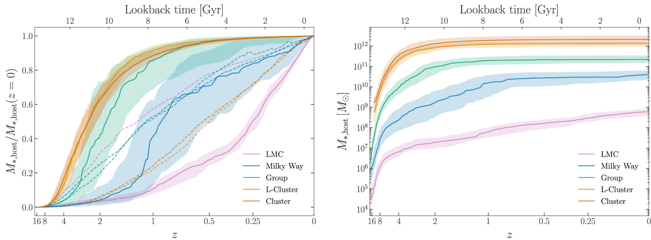
Figure 11. from Ethan O. Nadler et al 2023 Astrophys. J. 945 doi:10.3847/1538-4357/acb68c https://dx.doi.org/10.3847/1538-4357/acb68c © 2023. The Author(s). Published by the American Astronomical Society.
