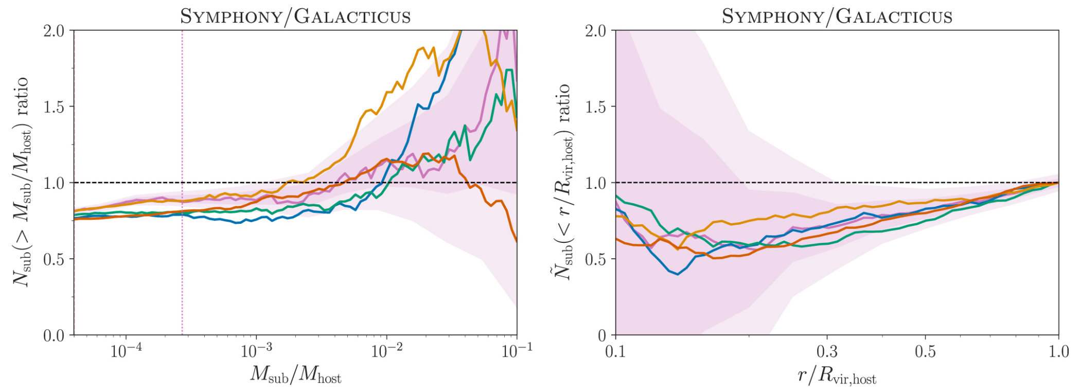
Figure 10. from Ethan O. Nadler et al 2023 Astrophys. J. 945 doi:10.3847/1538-4357/acb68c https://dx.doi.org/10.3847/1538-4357/acb68c © 2023. The Author(s). Published by the American Astronomical Society.
