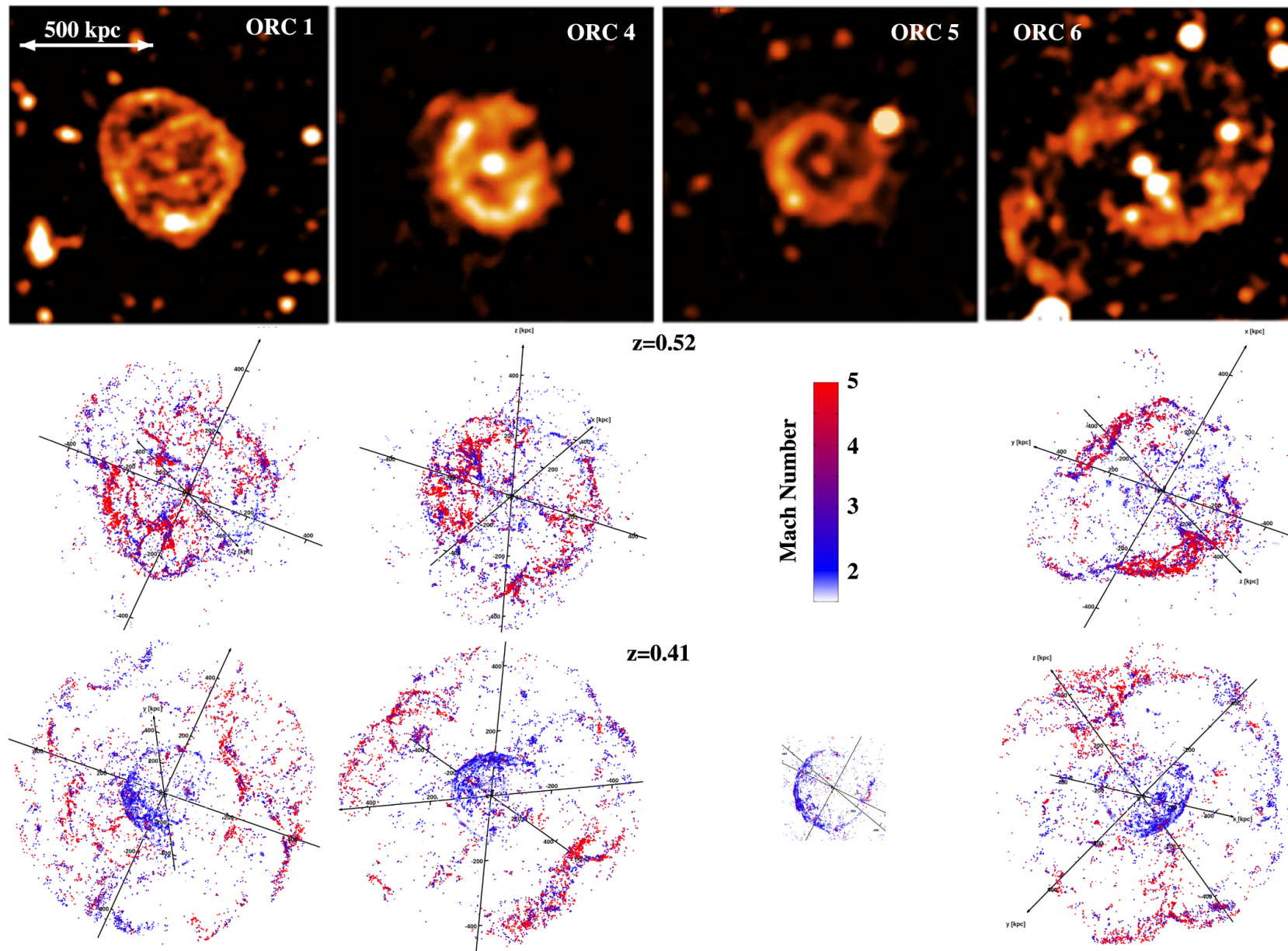
Figure 7. from Klaus Dolag et al 2023 Astrophys. J. 945 doi:10.3847/1538-4357/acb5f5 https://dx.doi.org/10.3847/1538-4357/acb5f5 © 2023. The Author(s). Published by the American Astronomical Society.
