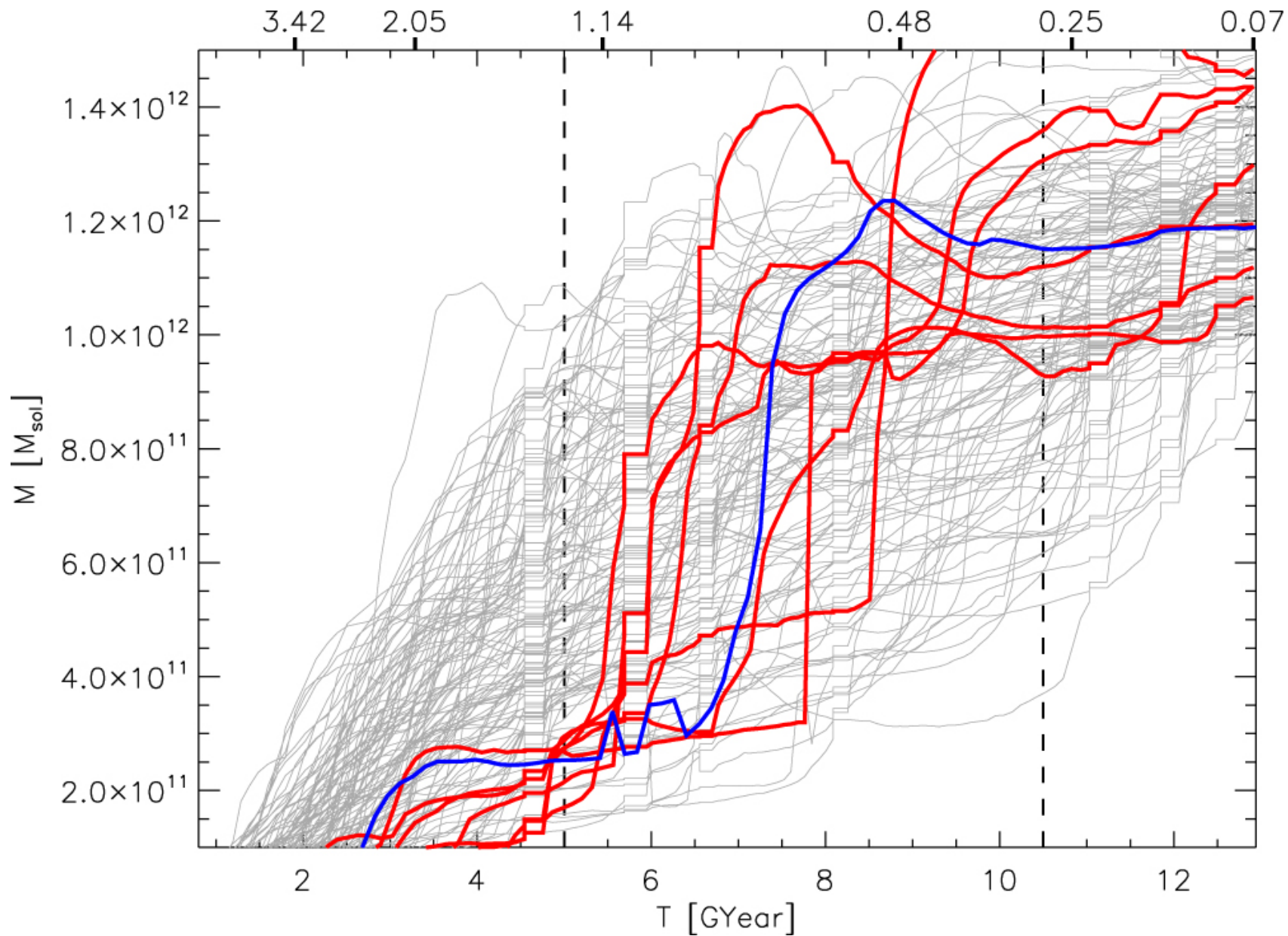
Figure 6. from Klaus Dolag et al 2023 Astrophys. J. 945 doi:10.3847/1538-4357/acb5f5 https://dx.doi.org/10.3847/1538-4357/acb5f5 © 2023. The Author(s). Published by the American Astronomical Society.
