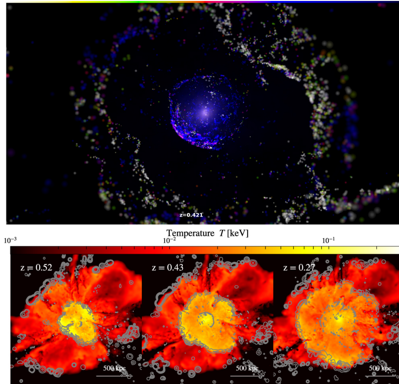
Figure 4. from Klaus Dolag et al 2023 Astrophys. J. 945 doi:10.3847/1538-4357/acb5f5 https://dx.doi.org/10.3847/1538-4357/acb5f5 © 2023. The Author(s). Published by the American Astronomical Society.
