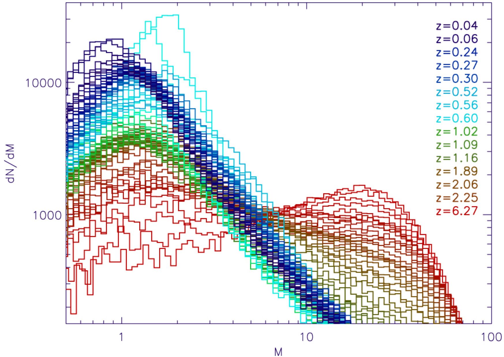
Figure 2. from Klaus Dolag et al 2023 Astrophys. J. 945 doi:10.3847/1538-4357/acb5f5 https://dx.doi.org/10.3847/1538-4357/acb5f5 © 2023. The Author(s). Published by the American Astronomical Society.
