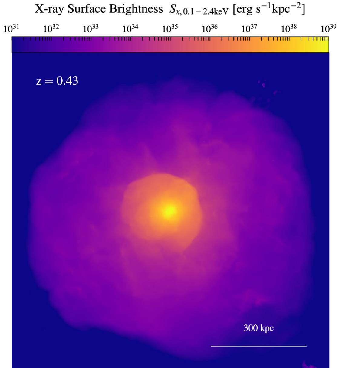
Figure 10. from Klaus Dolag et al 2023 Astrophys. J. 945 doi:10.3847/1538-4357/acb5f5 https://dx.doi.org/10.3847/1538-4357/acb5f5 © 2023. The Author(s). Published by the American Astronomical Society.
