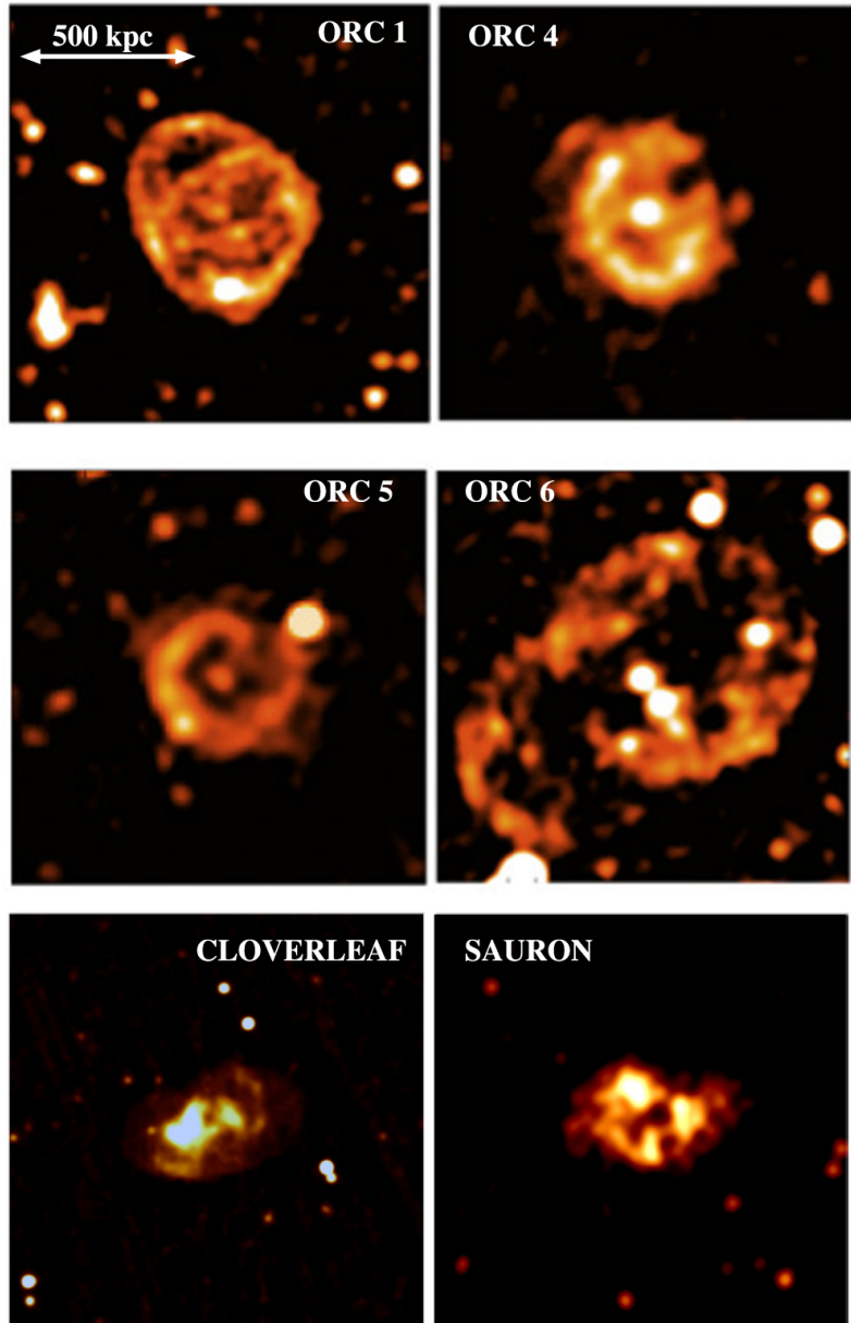
Figure 1. from Klaus Dolag et al 2023 Astrophys. J. 945 doi:10.3847/1538-4357/acb5f5 https://dx.doi.org/10.3847/1538-4357/acb5f5 © 2023. The Author(s). Published by the American Astronomical Society.
