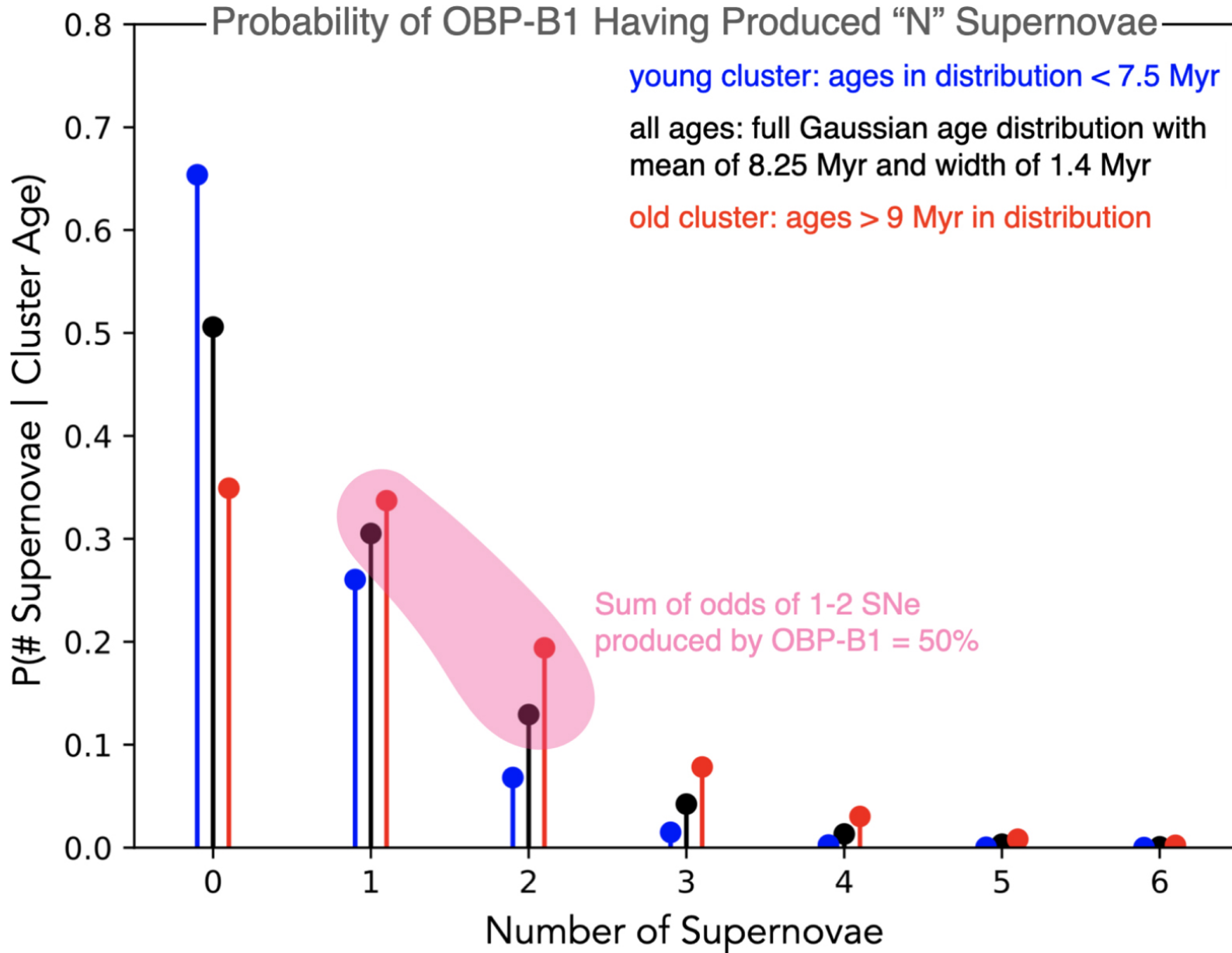
Figure 7. from Michael M. Foley et al 2023 Astrophys. J. 947 doi:10.3847/1538-4357/acb5f4 https://dx.doi.org/10.3847/1538-4357/acb5f4 © 2023. The Author(s). Published by the American Astronomical Society.
