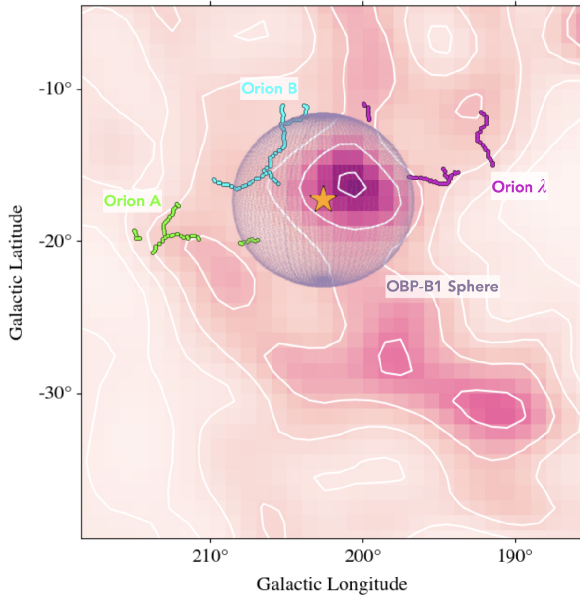
Figure 6. from Michael M. Foley et al 2023 Astrophys. J. 947 doi:10.3847/1538-4357/acb5f4 https://dx.doi.org/10.3847/1538-4357/acb5f4 © 2023. The Author(s). Published by the American Astronomical Society.
