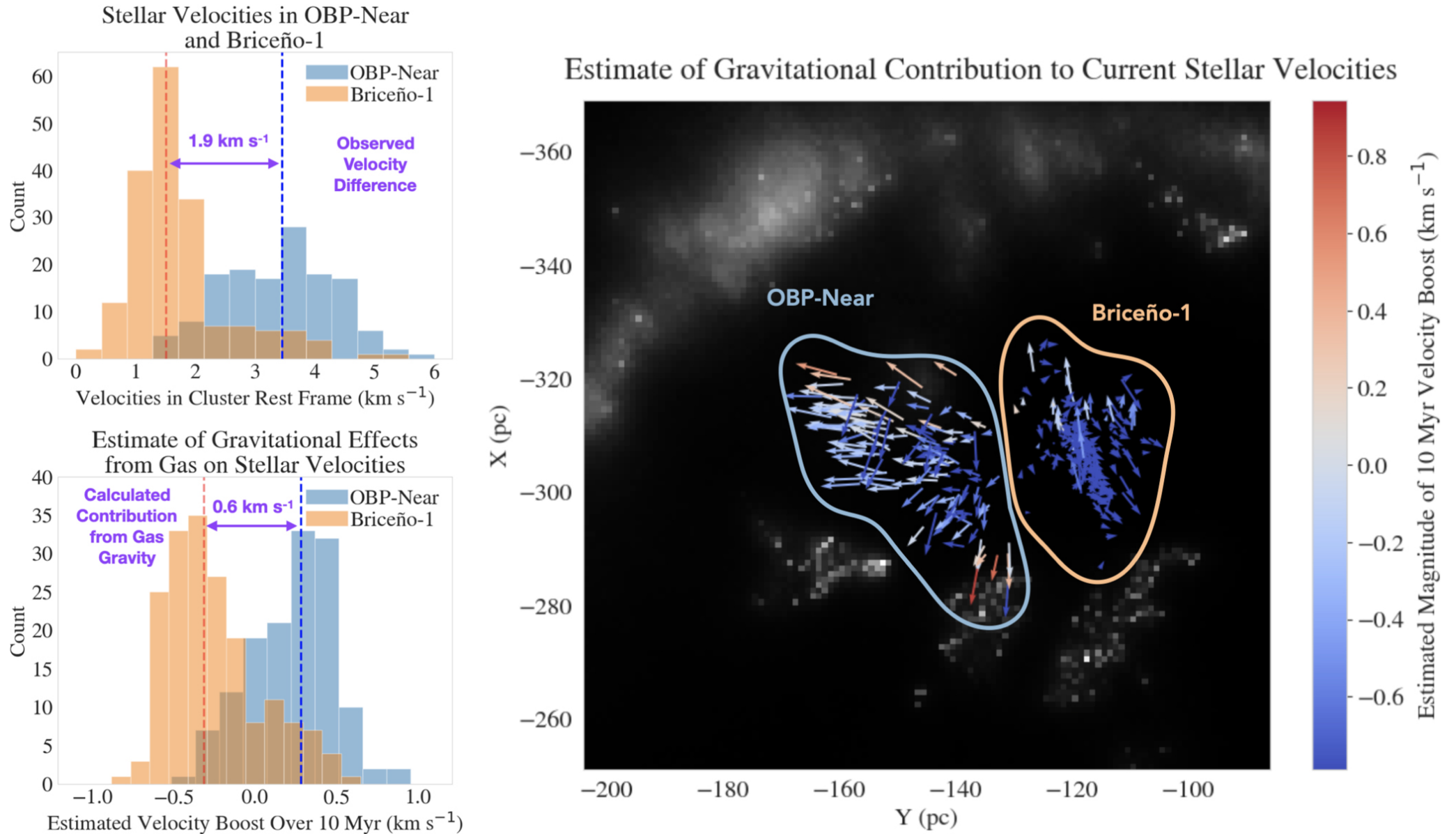
Figure 5. from Michael M. Foley et al 2023 Astrophys. J. 947 doi:10.3847/1538-4357/acb5f4 https://dx.doi.org/10.3847/1538-4357/acb5f4 © 2023. The Author(s). Published by the American Astronomical Society.
