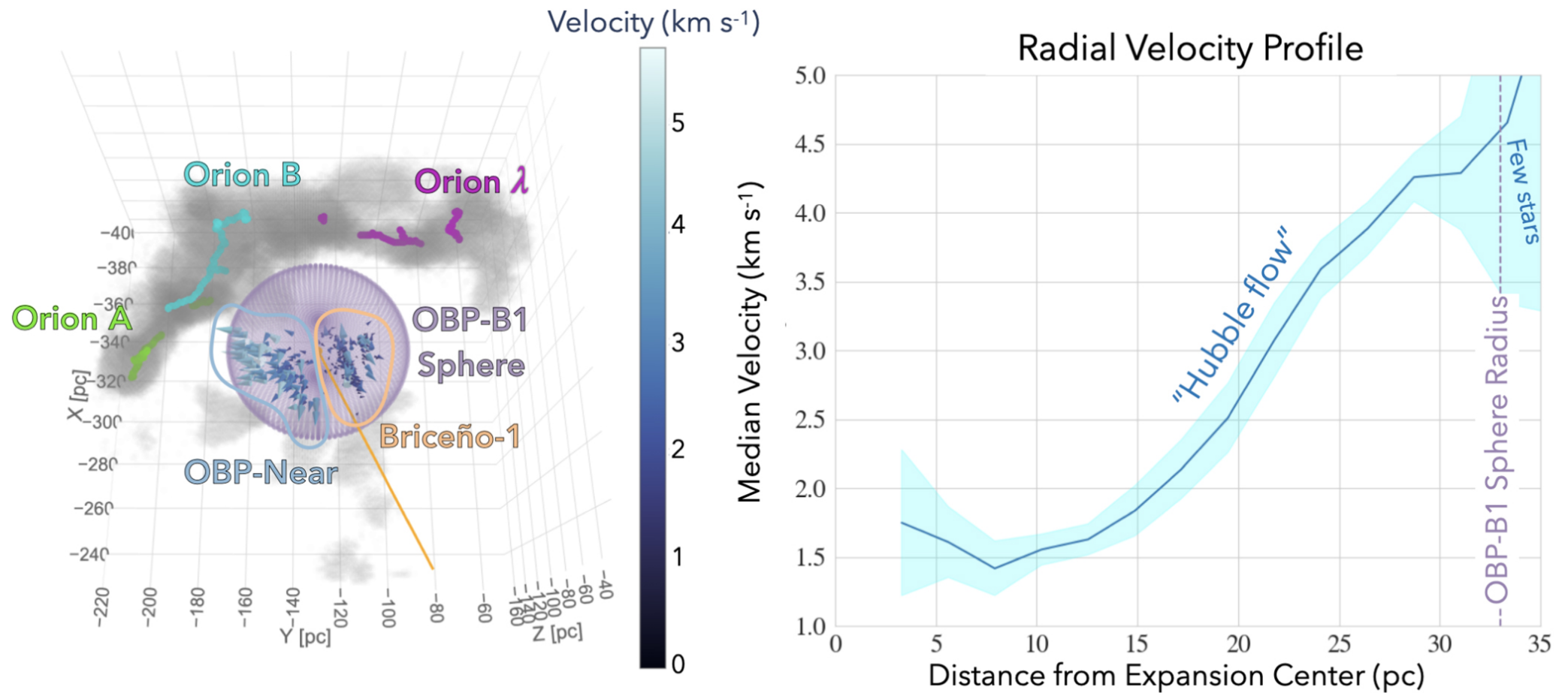
Figure 4. from Michael M. Foley et al 2023 Astrophys. J. 947 doi:10.3847/1538-4357/acb5f4 https://dx.doi.org/10.3847/1538-4357/acb5f4 © 2023. The Author(s). Published by the American Astronomical Society.
