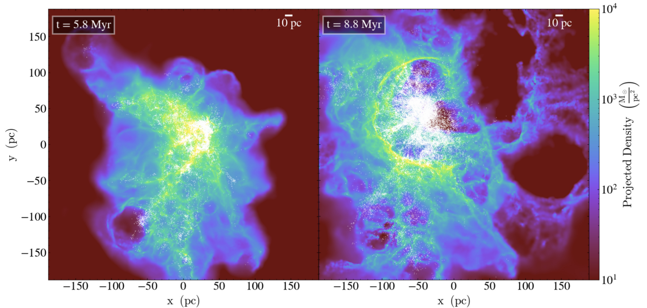
Figure 10. from Michael M. Foley et al 2023 Astrophys. J. 947 doi:10.3847/1538-4357/acb5f4 https://dx.doi.org/10.3847/1538-4357/acb5f4 © 2023. The Author(s). Published by the American Astronomical Society.
