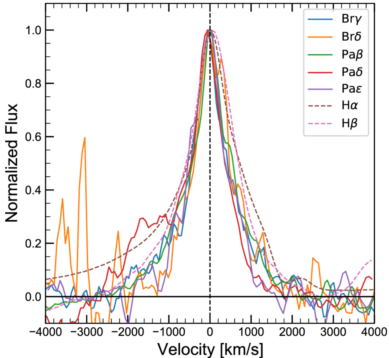
Figure 9. from Kohki Uno et al 2023 Astrophys. J. 944 doi:10.3847/1538-4357/acb5ec https://dx.doi.org/10.3847/1538-4357/acb5ec © 2023. The Author(s). Published by the American Astronomical Society.
