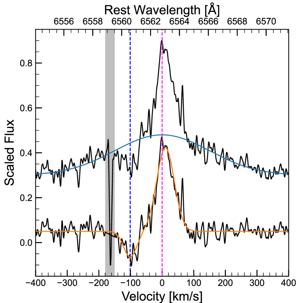
Figure 7. from Kohki Uno et al 2023 Astrophys. J. 944 doi:10.3847/1538-4357/acb5ec https://dx.doi.org/10.3847/1538-4357/acb5ec © 2023. The Author(s). Published by the American Astronomical Society.
