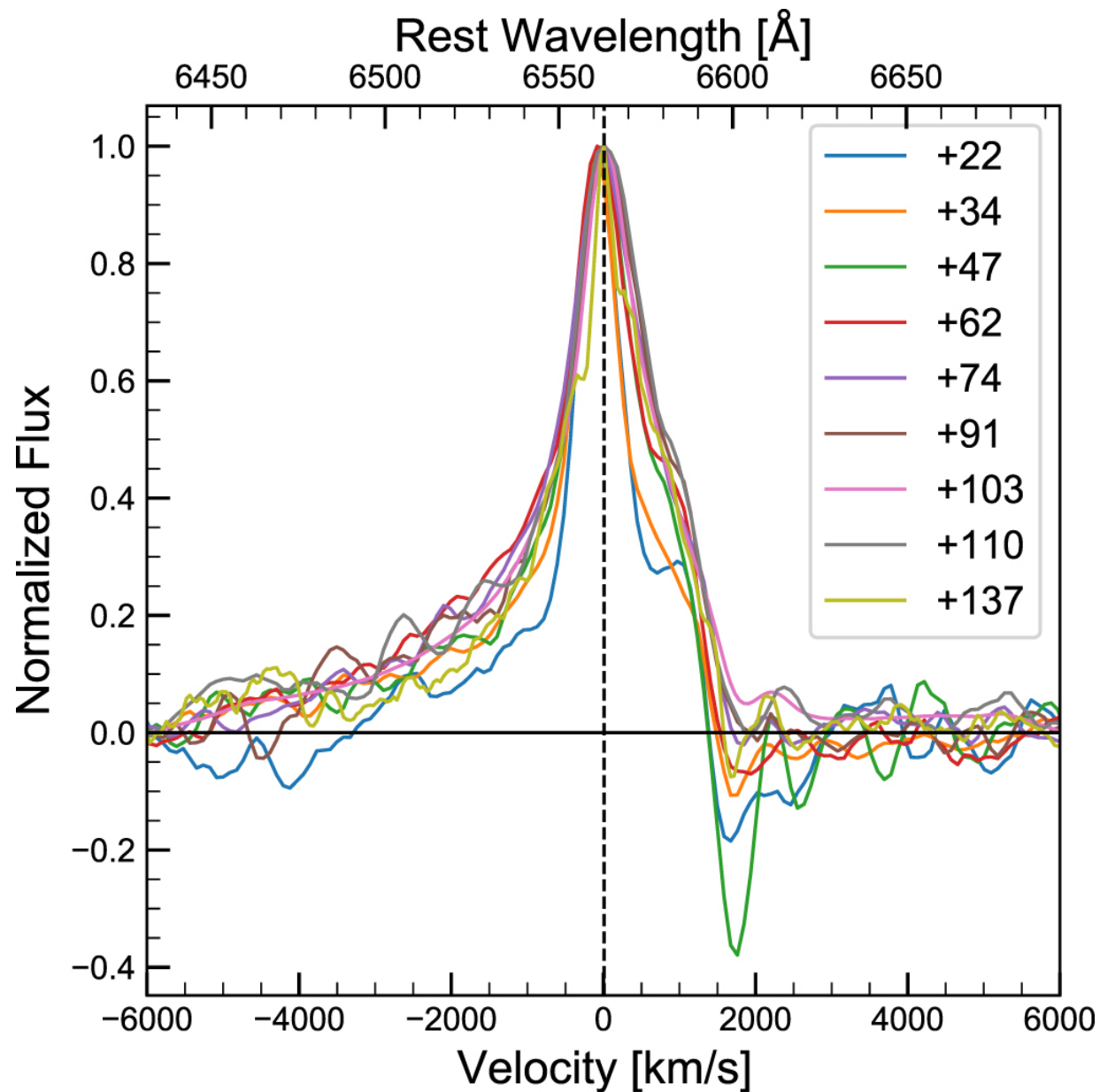
Figure 6. from Kohki Uno et al 2023 Astrophys. J. 944 doi:10.3847/1538-4357/acb5ec https://dx.doi.org/10.3847/1538-4357/acb5ec © 2023. The Author(s). Published by the American Astronomical Society.
