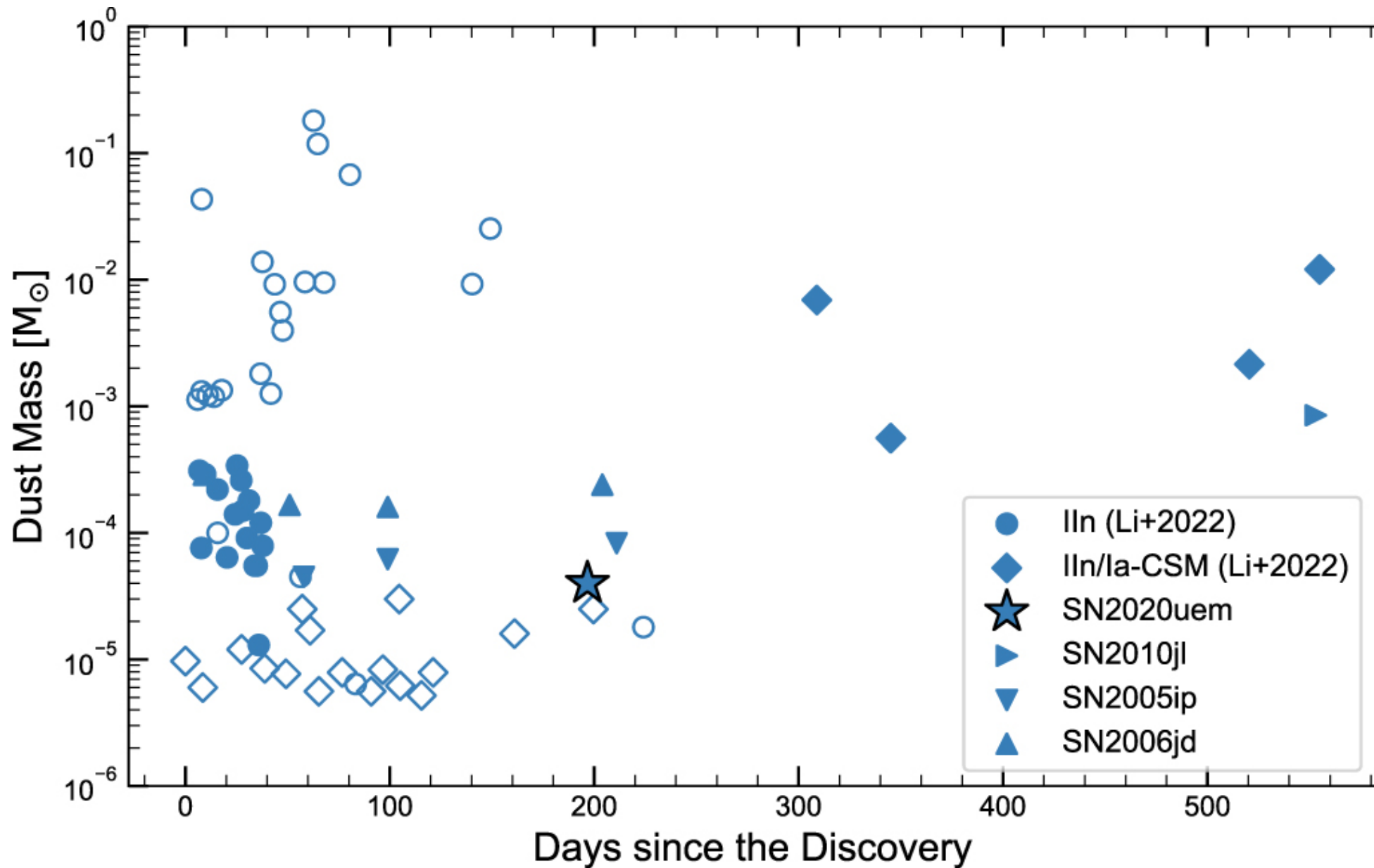
Figure 15. from Kohki Uno et al 2023 Astrophys. J. 944 doi:10.3847/1538-4357/acb5ec https://dx.doi.org/10.3847/1538-4357/acb5ec © 2023. The Author(s). Published by the American Astronomical Society.
