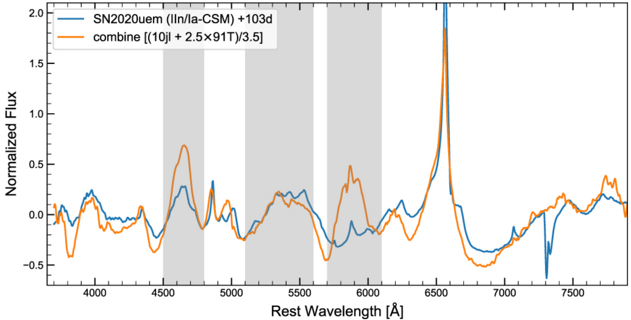
Figure 14. from Kohki Uno et al 2023 Astrophys. J. 944 doi:10.3847/1538-4357/acb5ec https://dx.doi.org/10.3847/1538-4357/acb5ec © 2023. The Author(s). Published by the American Astronomical Society.
