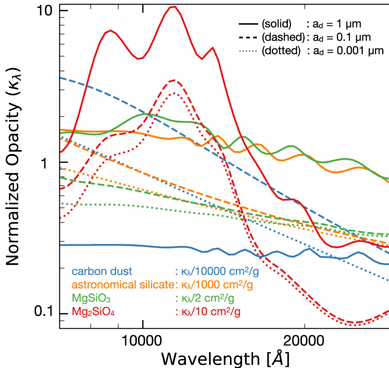
Figure 10. from Kohki Uno et al 2023 Astrophys. J. 944 doi:10.3847/1538-4357/acb5ec https://dx.doi.org/10.3847/1538-4357/acb5ec © 2023. The Author(s). Published by the American Astronomical Society.
