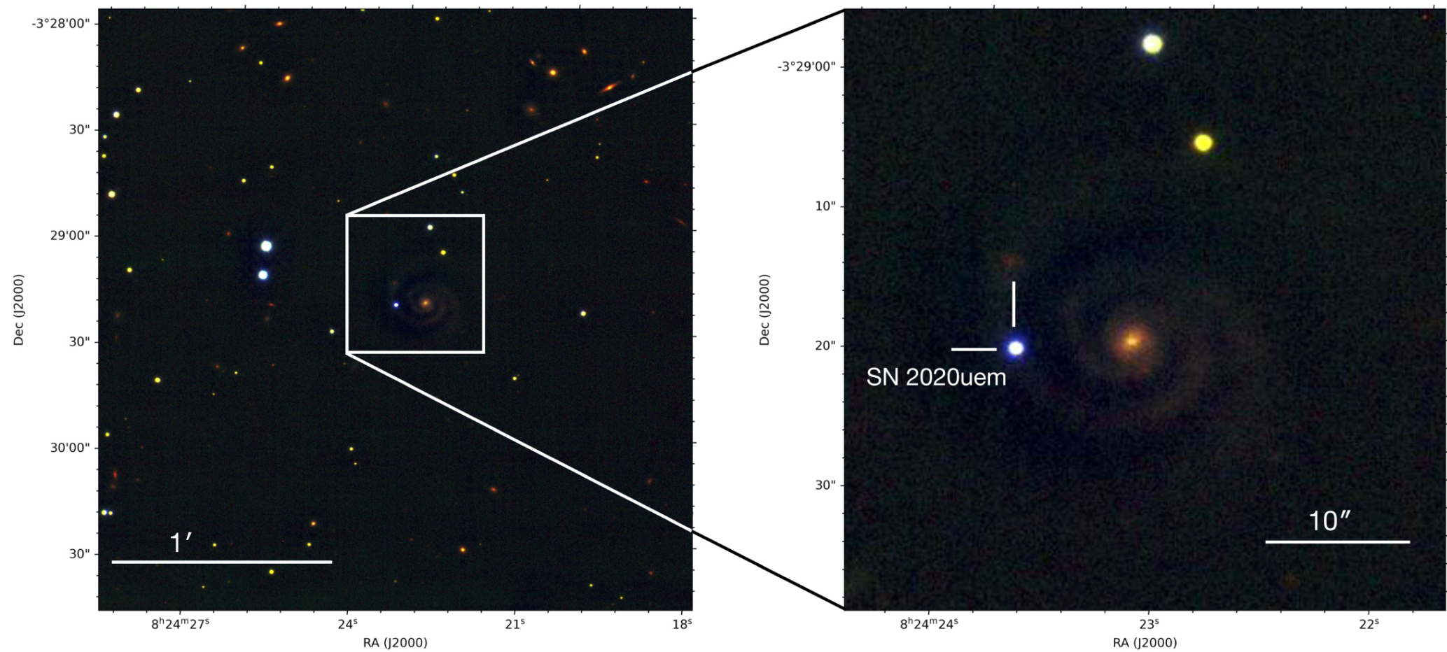
Figure 1. from Kohki Uno et al 2023 Astrophys. J. 944 doi:10.3847/1538-4357/acb5ec https://dx.doi.org/10.3847/1538-4357/acb5ec © 2023. The Author(s). Published by the American Astronomical Society.
