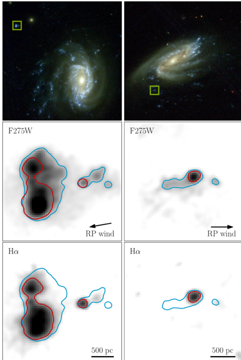
Figure 7. from Marco Gullieuszik et al 2023 Astrophys. J. 945 doi:10.3847/1538-4357/acb59b https://dx.doi.org/10.3847/1538-4357/acb59b © 2023. The Author(s). Published by the American Astronomical Society.
