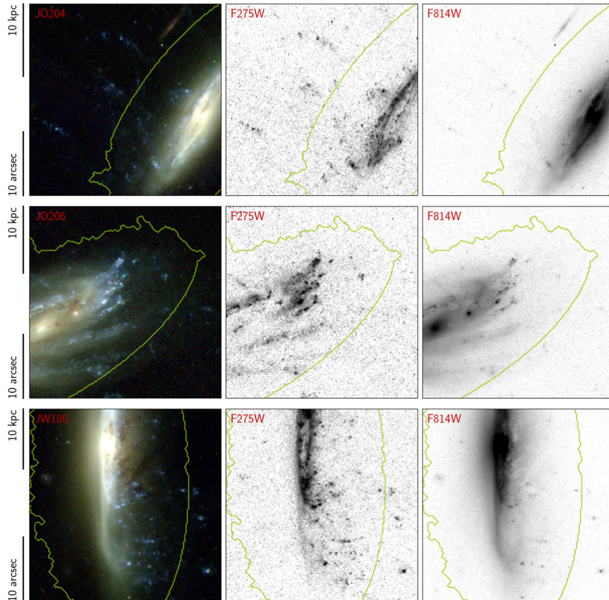
Figure 6. from Marco Gullieuszik et al 2023 Astrophys. J. 945 doi:10.3847/1538-4357/acb59b https://dx.doi.org/10.3847/1538-4357/acb59b © 2023. The Author(s). Published by the American Astronomical Society.
