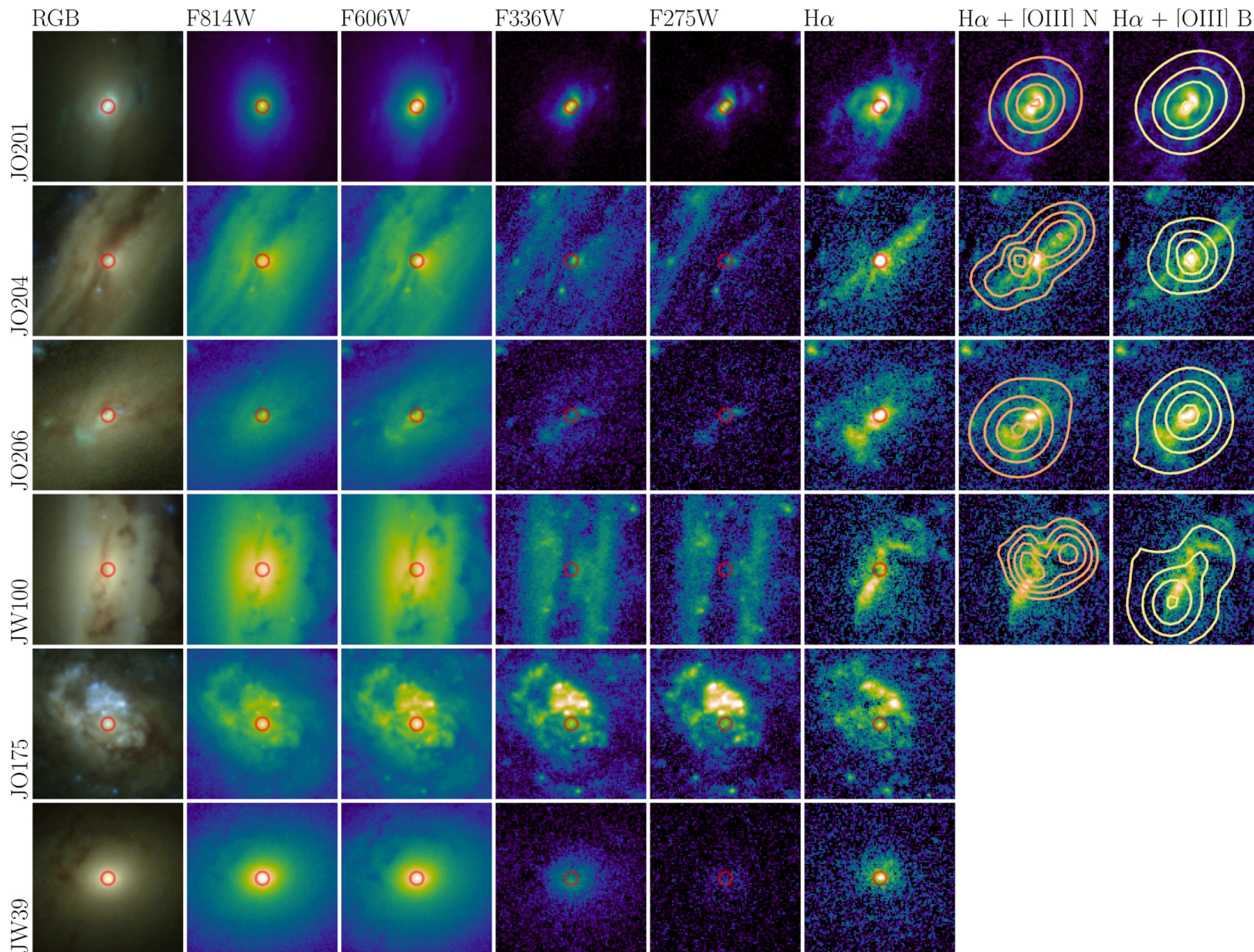
Figure 5. from Marco Gullieuszik et al 2023 Astrophys. J. 945 doi:10.3847/1538-4357/acb59b https://dx.doi.org/10.3847/1538-4357/acb59b © 2023. The Author(s). Published by the American Astronomical Society.
