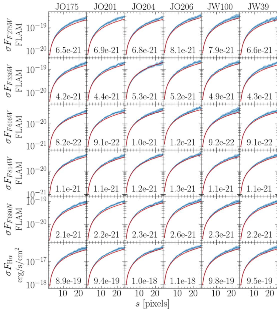
Figure 4. from Marco Gullieuszik et al 2023 Astrophys. J. 945 doi:10.3847/1538-4357/acb59b https://dx.doi.org/10.3847/1538-4357/acb59b © 2023. The Author(s). Published by the American Astronomical Society.
