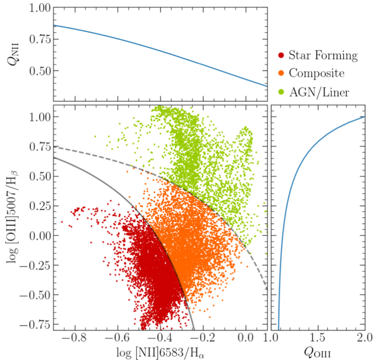
Figure 2. from Marco Gullieuszik et al 2023 Astrophys. J. 945 doi:10.3847/1538-4357/acb59b https://dx.doi.org/10.3847/1538-4357/acb59b © 2023. The Author(s). Published by the American Astronomical Society.
