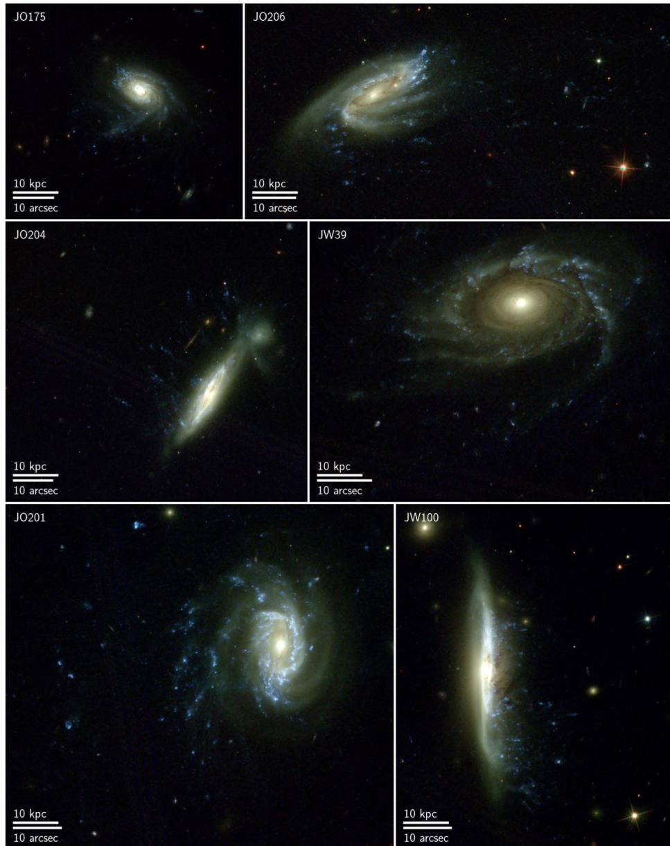
Figure 1. from Marco Gullieuszik et al 2023 Astrophys. J. 945 doi:10.3847/1538-4357/acb59b https://dx.doi.org/10.3847/1538-4357/acb59b © 2023. The Author(s). Published by the American Astronomical Society.
