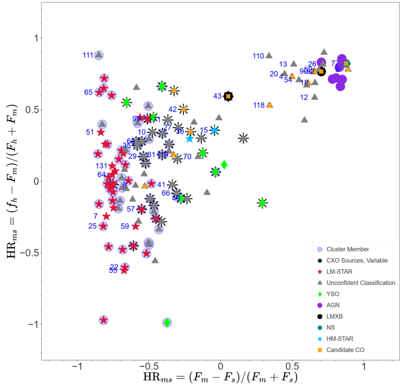
Figure 9. from Steven Chen et al 2023 Astrophys. J. 948 doi:10.3847/1538-4357/acb3a6 https://dx.doi.org/10.3847/1538-4357/acb3a6 © 2023. The Author(s). Published by the American Astronomical Society.
