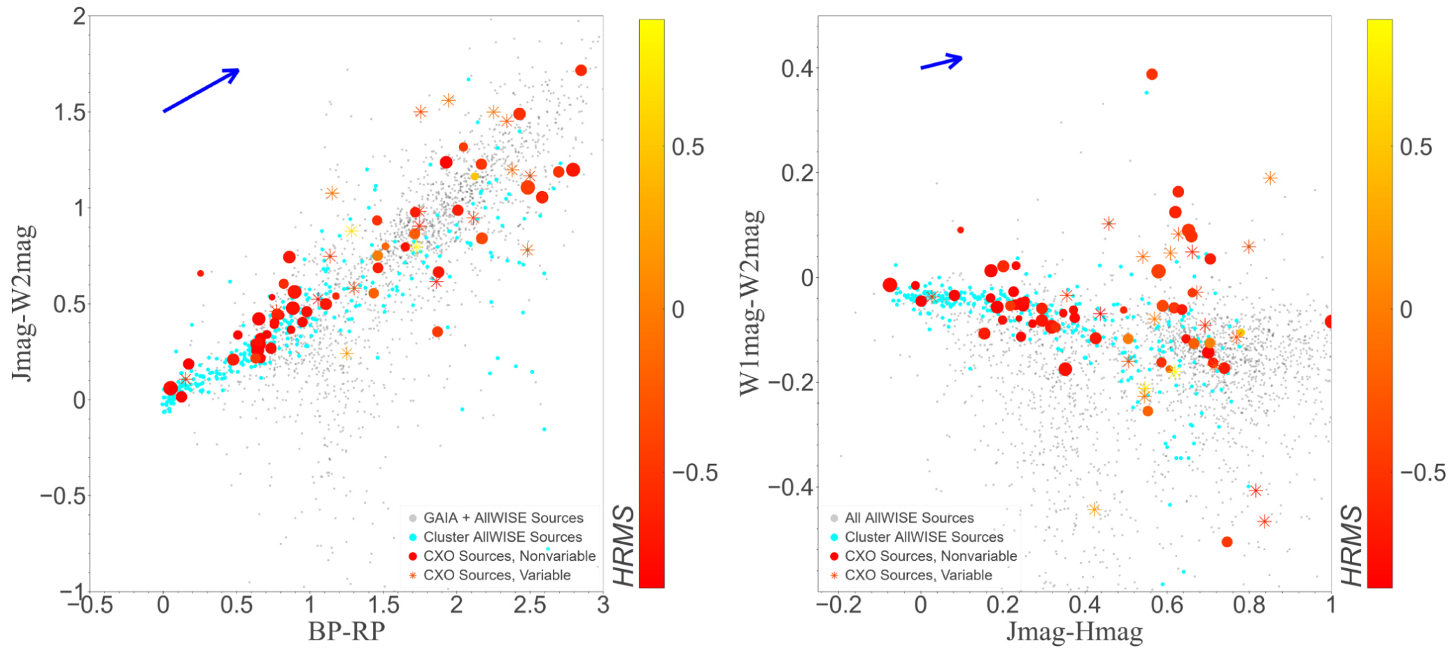
Figure 6. from Steven Chen et al 2023 Astrophys. J. 948 doi:10.3847/1538-4357/acb3a6 https://dx.doi.org/10.3847/1538-4357/acb3a6 © 2023. The Author(s). Published by the American Astronomical Society.
