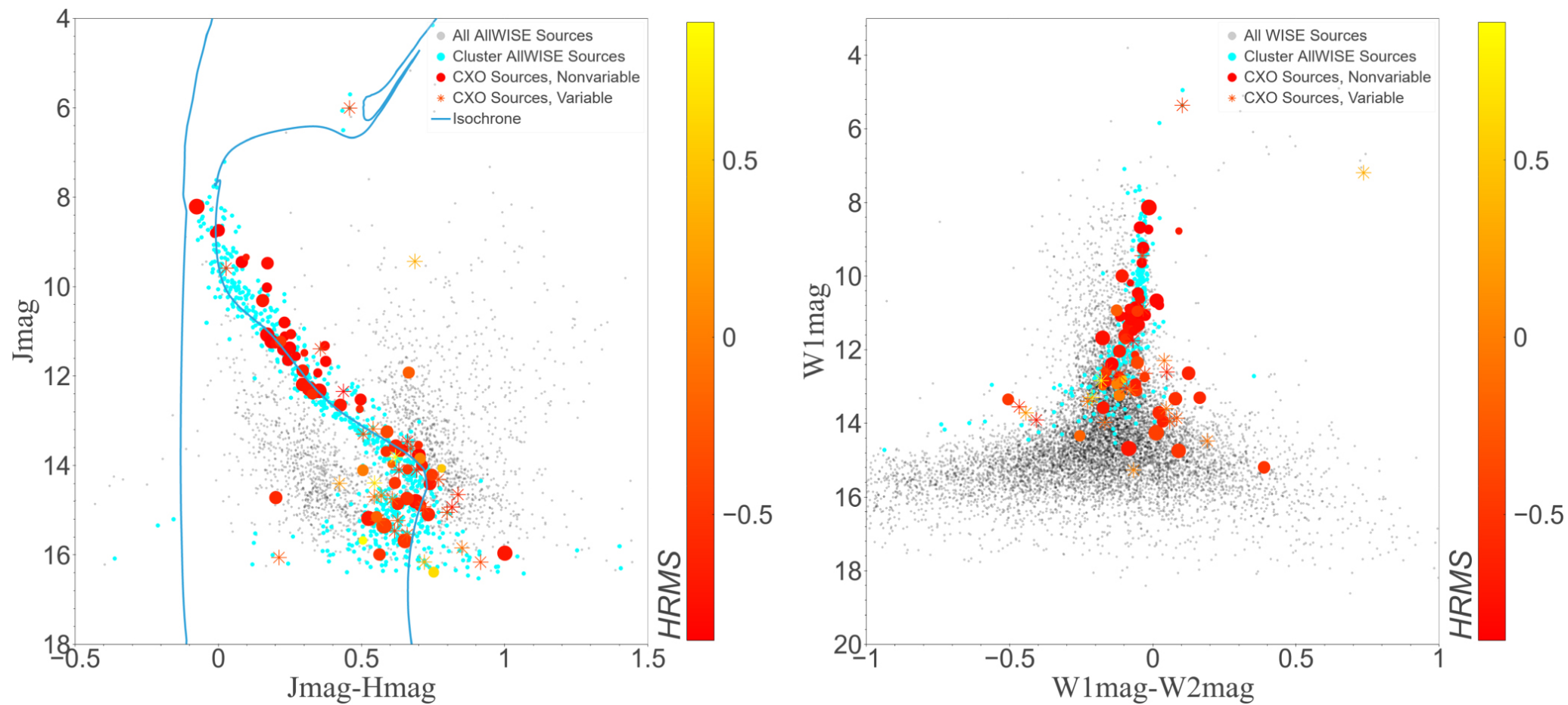
Figure 4. from Steven Chen et al 2023 Astrophys. J. 948 doi:10.3847/1538-4357/acb3a6 https://dx.doi.org/10.3847/1538-4357/acb3a6 © 2023. The Author(s). Published by the American Astronomical Society.
