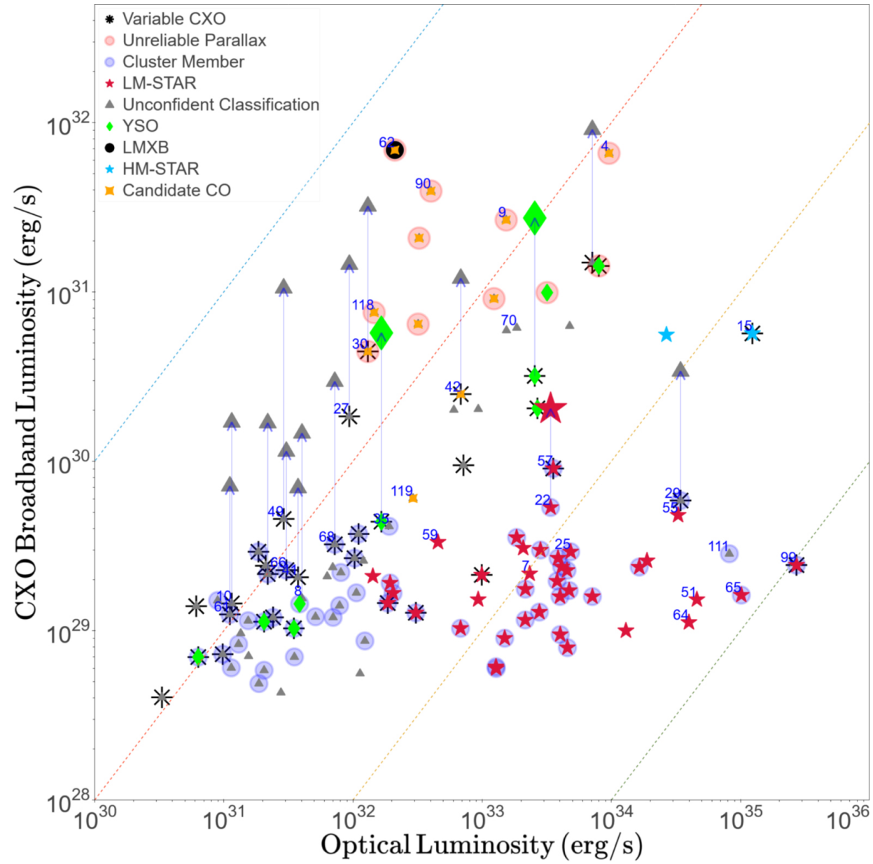
Figure 11. from Steven Chen et al 2023 Astrophys. J. 948 doi:10.3847/1538-4357/acb3a6 https://dx.doi.org/10.3847/1538-4357/acb3a6 © 2023. The Author(s). Published by the American Astronomical Society.
