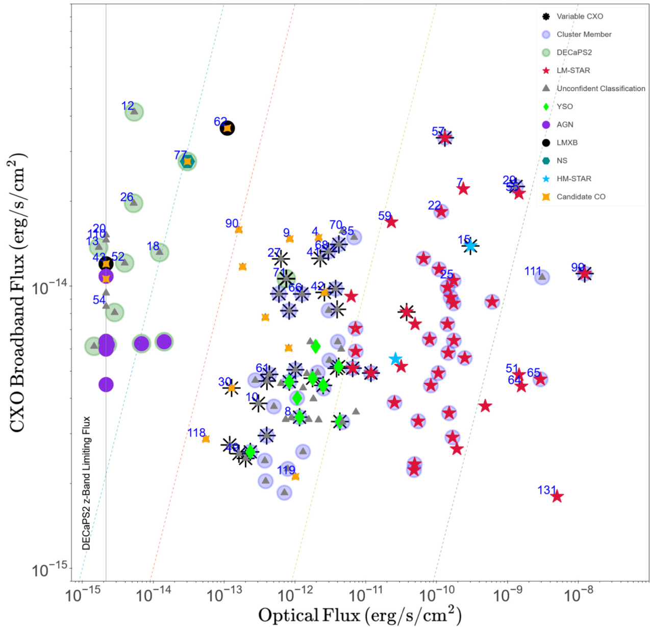
Figure 10. from Steven Chen et al 2023 Astrophys. J. 948 doi:10.3847/1538-4357/acb3a6 https://dx.doi.org/10.3847/1538-4357/acb3a6 © 2023. The Author(s). Published by the American Astronomical Society.
