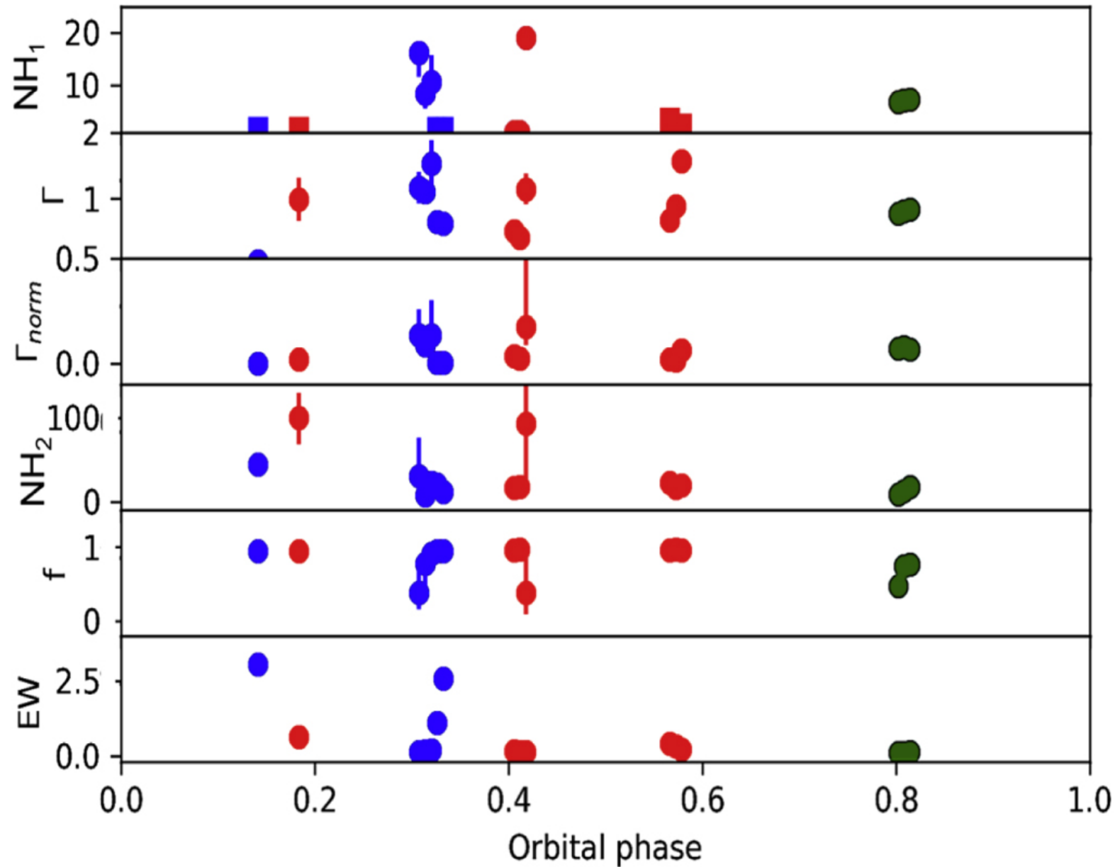
Figure 9. from Pragati Pradhan et al 2023 Astrophys. J. 945 doi:10.3847/1538-4357/acb2cb https://dx.doi.org/10.3847/1538-4357/acb2cb © 2023. The Author(s). Published by the American Astronomical Society.
