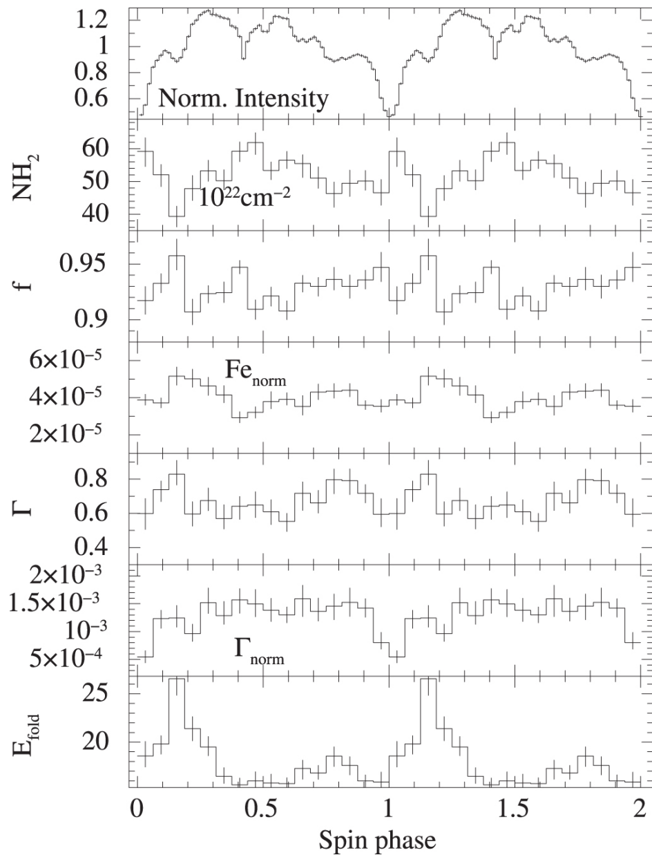
Figure 7. from Pragati Pradhan et al 2023 Astrophys. J. 945 doi:10.3847/1538-4357/acb2cb https://dx.doi.org/10.3847/1538-4357/acb2cb © 2023. The Author(s). Published by the American Astronomical Society.
