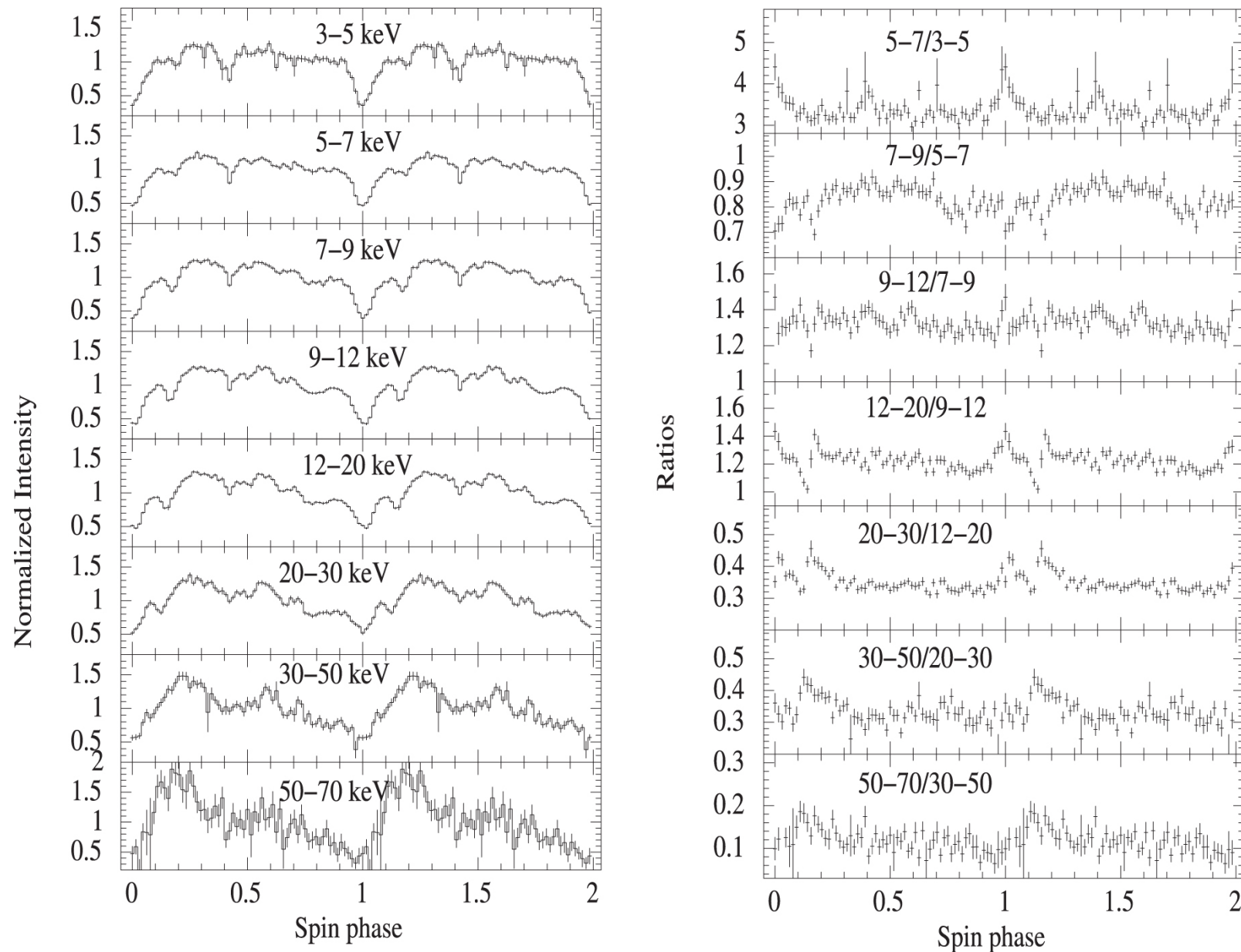
Figure 6. from Pragati Pradhan et al 2023 Astrophys. J. 945 doi:10.3847/1538-4357/acb2cb https://dx.doi.org/10.3847/1538-4357/acb2cb © 2023. The Author(s). Published by the American Astronomical Society.
