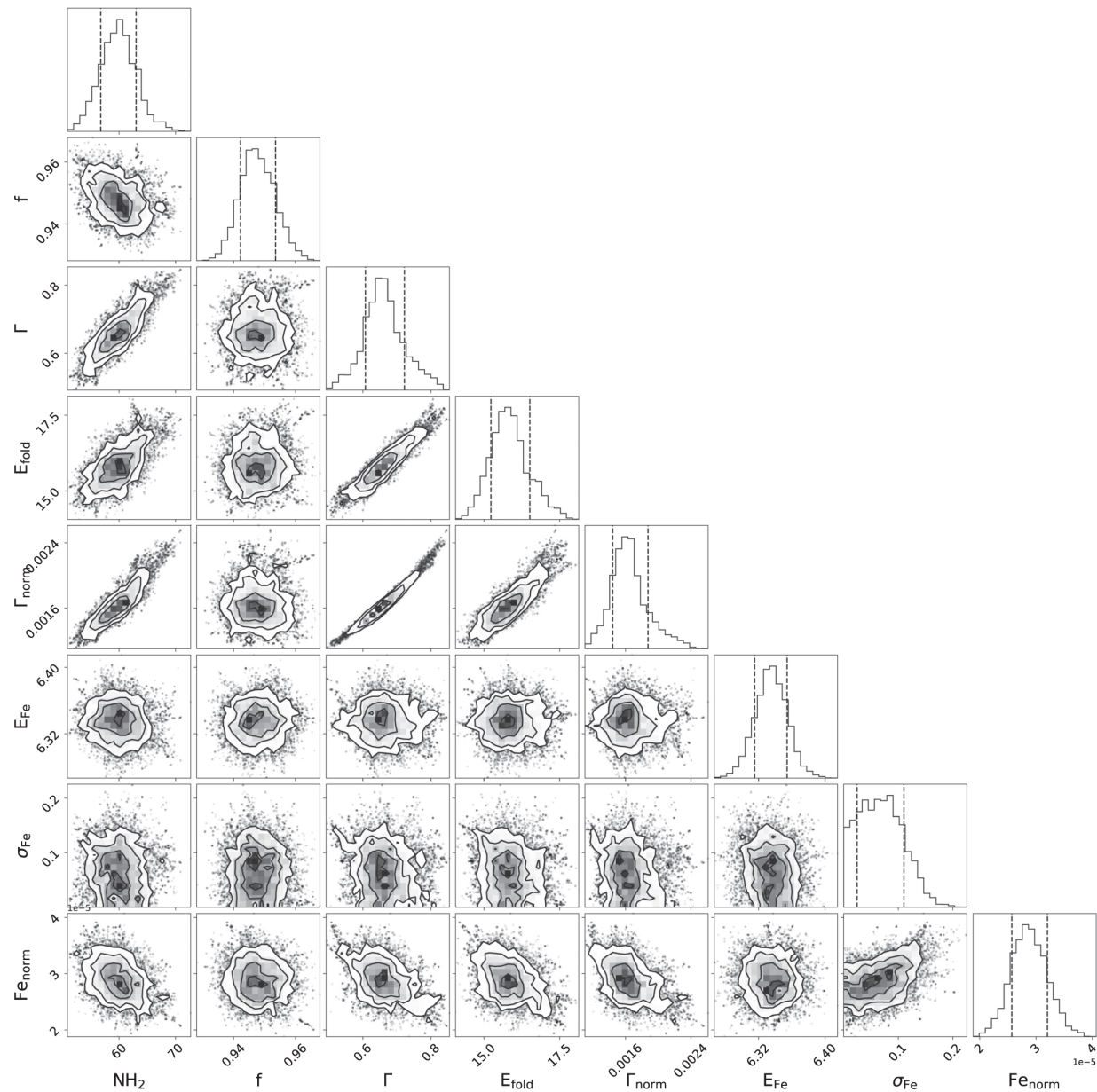
Figure A6. from Pragati Pradhan et al 2023 Astrophys. J. 945 doi:10.3847/1538-4357/acb2cb https://dx.doi.org/10.3847/1538-4357/acb2cb © 2023. The Author(s). Published by the American Astronomical Society.
