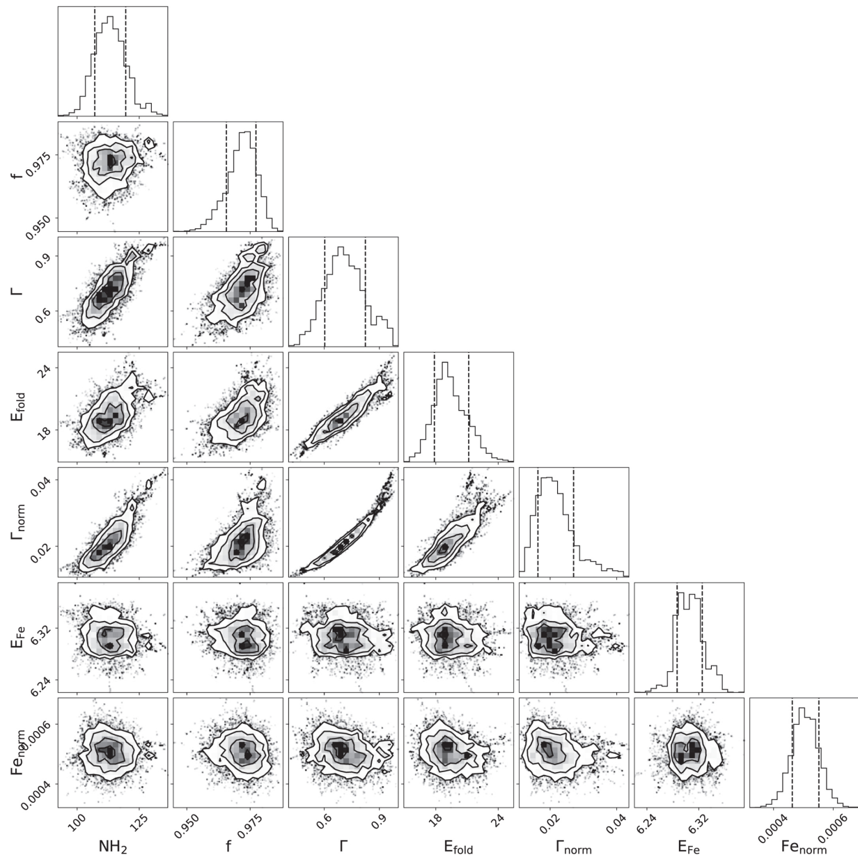
Figure A4. from Pragati Pradhan et al 2023 Astrophys. J. 945 doi:10.3847/1538-4357/acb2cb https://dx.doi.org/10.3847/1538-4357/acb2cb © 2023. The Author(s). Published by the American Astronomical Society.
