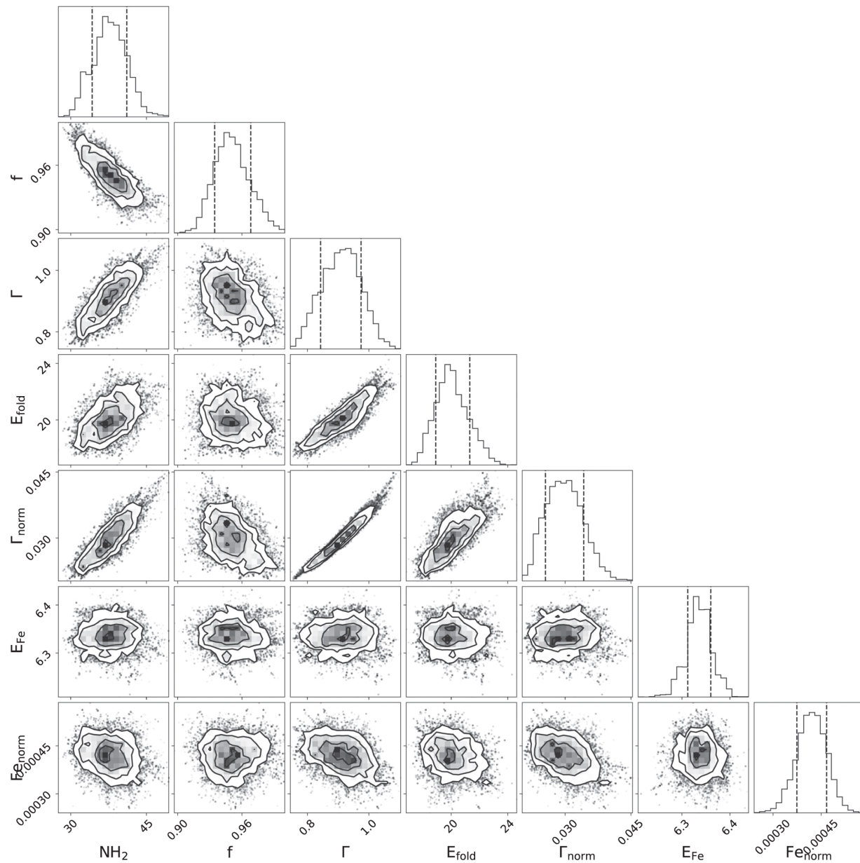
Figure A3. from Pragati Pradhan et al 2023 Astrophys. J. 945 doi:10.3847/1538-4357/acb2cb https://dx.doi.org/10.3847/1538-4357/acb2cb © 2023. The Author(s). Published by the American Astronomical Society.
