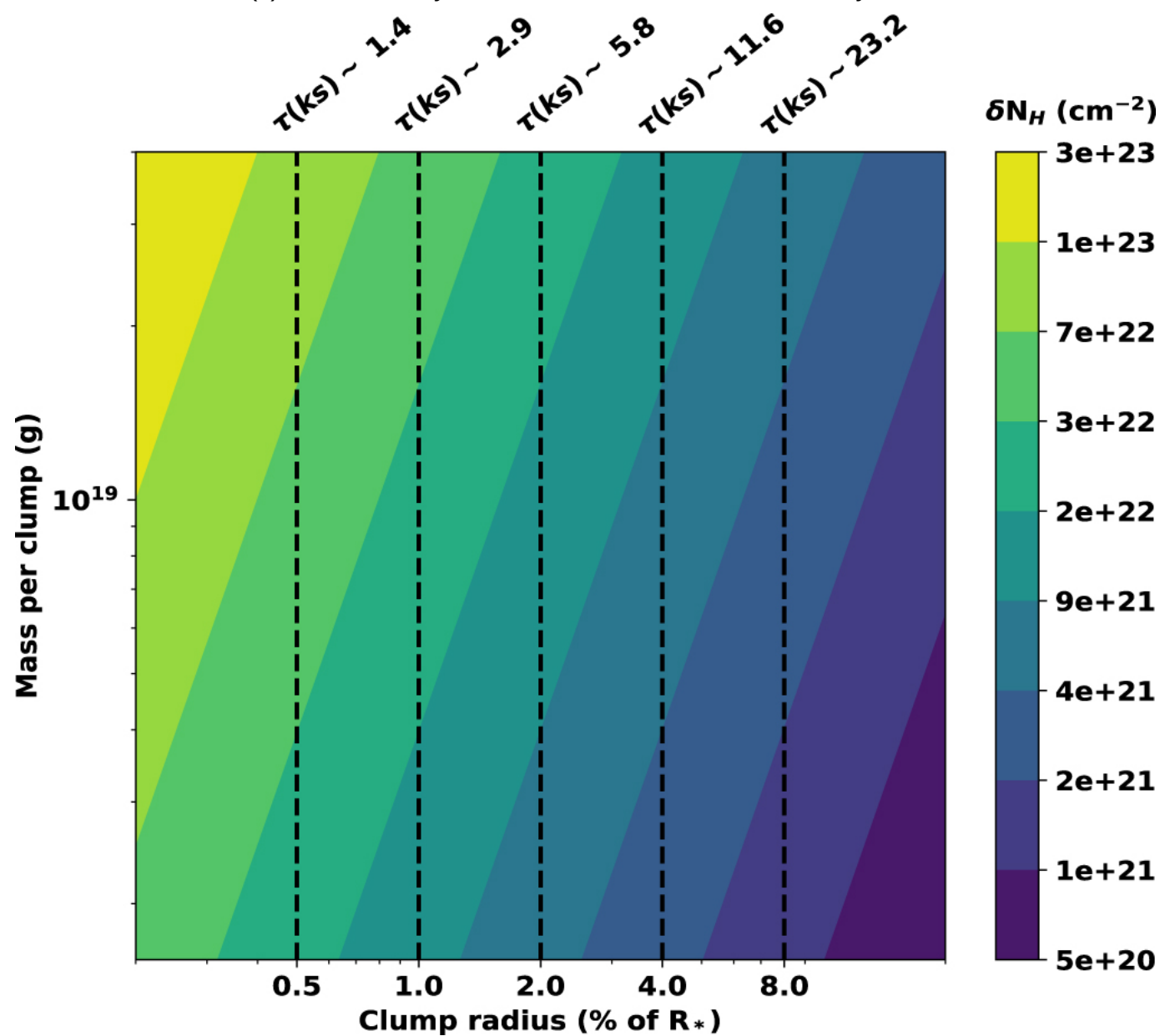
Figure 11. from Pragati Pradhan et al 2023 Astrophys. J. 945 doi:10.3847/1538-4357/acb2cb https://dx.doi.org/10.3847/1538-4357/acb2cb © 2023. The Author(s). Published by the American Astronomical Society.
