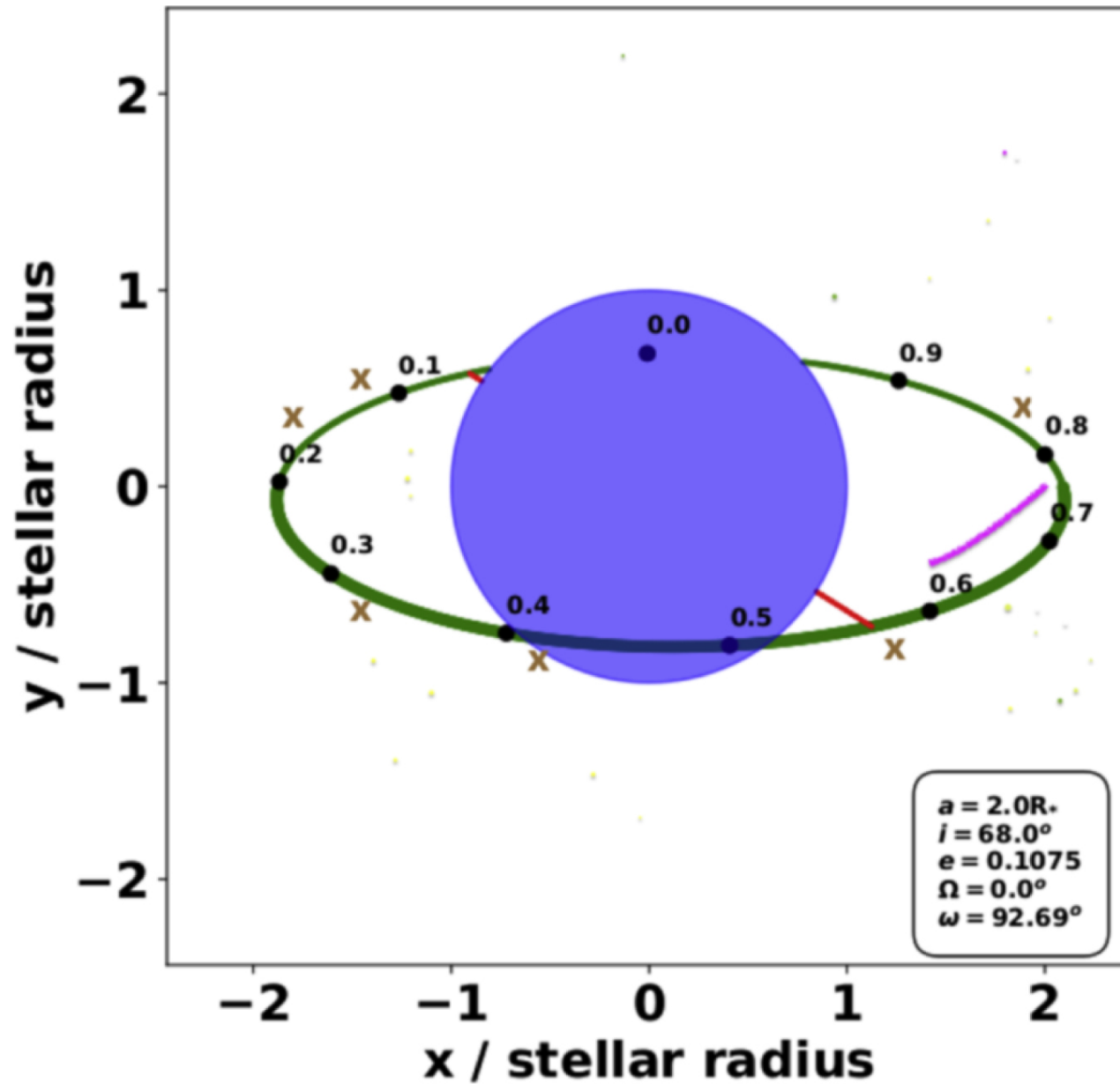
Figure 1. from Pragati Pradhan et al 2023 Astrophys. J. 945 doi:10.3847/1538-4357/acb2cb https://dx.doi.org/10.3847/1538-4357/acb2cb © 2023. The Author(s). Published by the American Astronomical Society.
